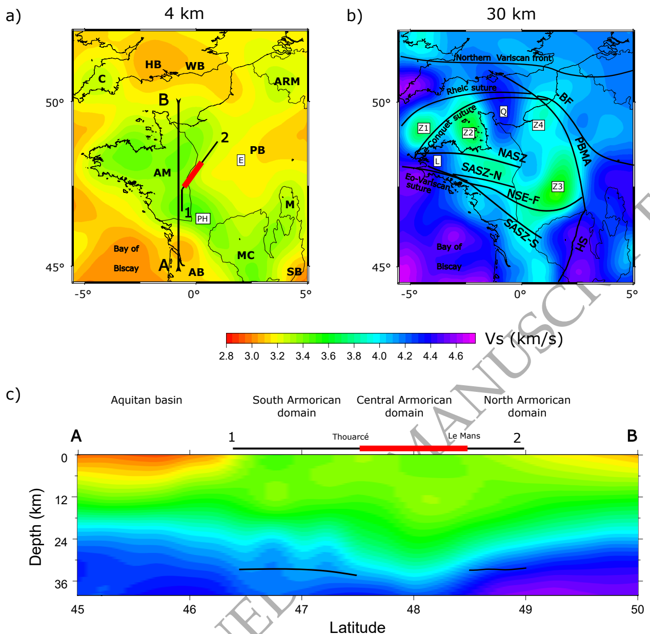
Figure 9. Isotropic V_S horizontal and vertical cross-section in the 3-D model for western France and the surrounding regions. a) 4 km horizontal cross-section. The position of the vertical cross-section presented in c) is indicated with A and B. The position of the ECORS profile [Matte & Hirn, 1988] is indicated with 1 and 2. b) 30 km horizontal cross-section. See Figure 1a for legend. Labelled white rectangles indicate specific features discussed in the text. c) Vertical cross-section at -1° longitude between 45° and 50° latitude. The continuous black lines superimposed on the section report the Moho depth detected along the ECORS profile. The red rectangle indicates the area between the cities of Thouarcé and Le Mans where anomalous reflectivity and attenuation pattern have been detected [Matte & Hirn, 1988; Campillo & Plantet, 1991]. See text for details.
