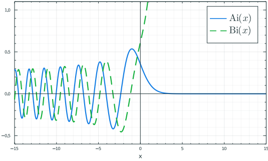
(A) Airy functions Ai and Bi.
