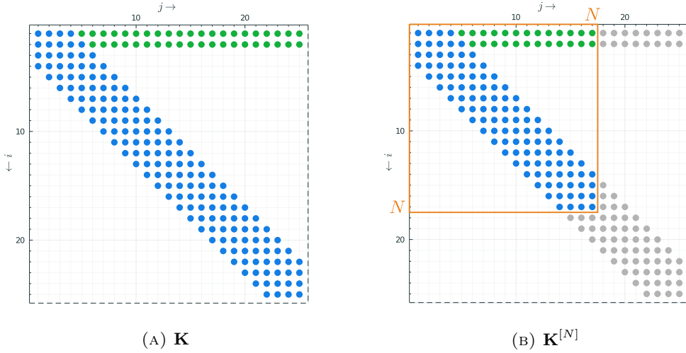
FIGURE 1. Almost-banded matrix representations in the Chebyshev basis of an integral operator \mathbf{K} and its truncation \mathbf{K}^{[N]} .
