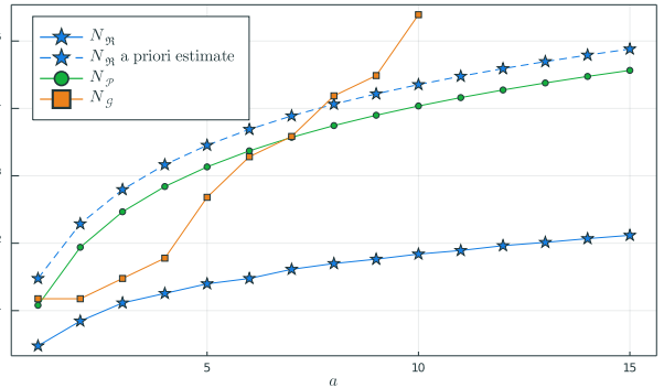
(D) Comparison of Newton-Picard's N_{\mathfrak{NP}} (real value and a priori estimate) with Newton-Galerkin's N_G and the number N_{\mathcal{P}} of Picard iterations in [2].
