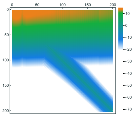
(C) (\mathbf{I} + \mathbf{K})^{-1} with \mathbf{K} in (24) and a = 15 .
