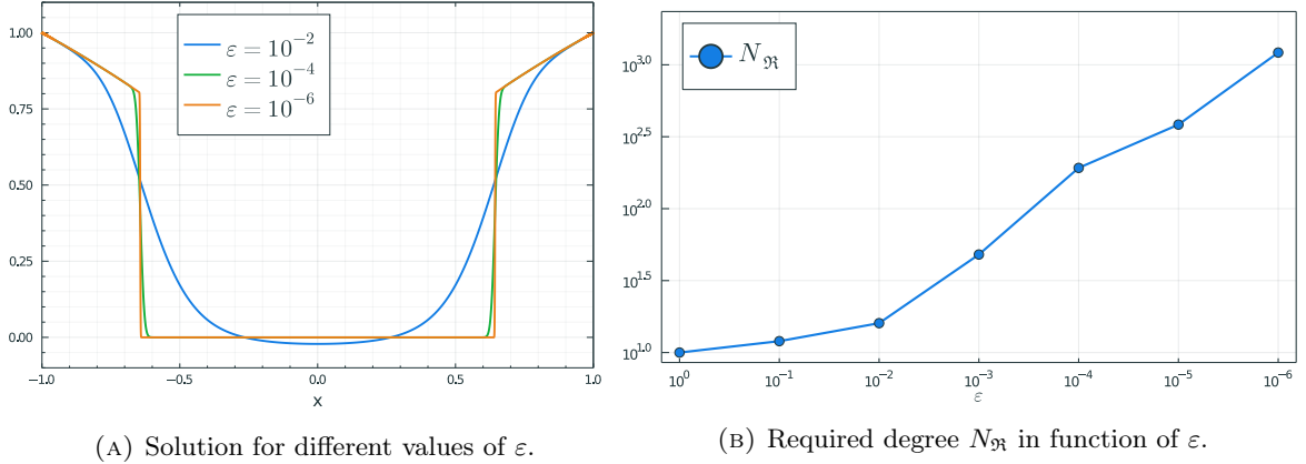
FIGURE 4. Validation of the boundary layer example using NEWTONPICARDVALID.
