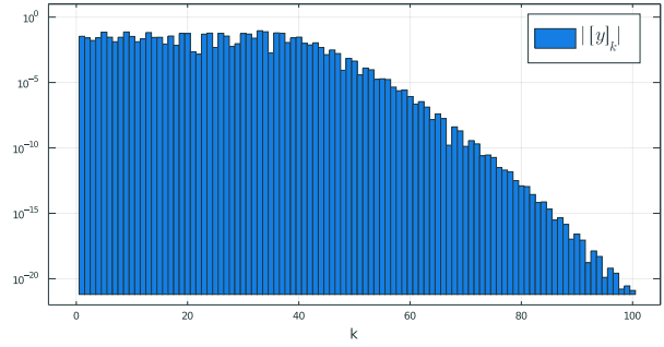
(B) Chebyshev coefficients of y = \text{Ai} for a = 15 .
