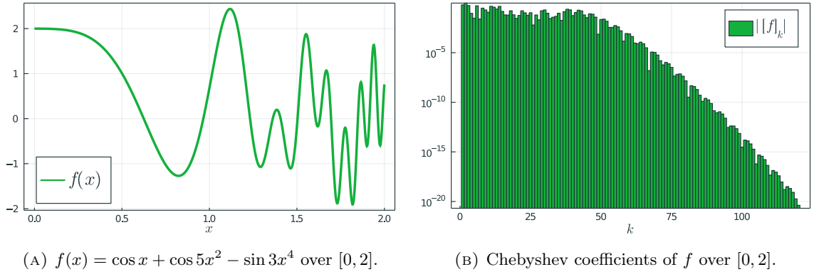
FIGURE 5. An example of a D-finite function with high-order, ill-conditioned differential equation.
