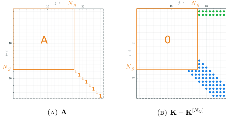
FIGURE 2. Bounding the truncation error \|\mathbf{A}(\mathbf{K} - \mathbf{K}^{[N_G]})\|_{\mathfrak{U}^1} in Newton-Galerkin method.
