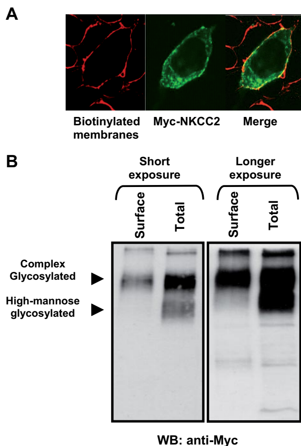
FIGURE 2. NKCC2 surface expression. A , immunolocalization of Myc-NKCC2. MKTAL cells membranes were biotinylated at 4 °C. Then the monolayers were fixed and stained for Myc-NKCC2 fusion protein (Cy-2) and cell surface biotin (avidin-Cy3). The stained specimens were evaluated by confocal microscopy. Optical sections (XY) at the cell surface are depicted for the Cy2 channel (green), Cy3 channel (red), and a merged channel. The yellow color indicates that Myc-NKCC-2 co-localizes with biotinylated proteins in the cell surface indicating adequate targeting of the co-transporter to the plasma membrane. B , confluent cells were biotinylated at 4 °C with the cleavable biotinylation reagent sulfo-NHS-SS-biotin. Biotinylated proteins were recovered from cell extracts by precipitation with streptavidin-agarose. NKCC2 on the cell surface was detected by Western blotting with Myc antibody. An aliquot of the total cell extract from each sample was also run on a parallel SDS gel and Western blotted (WB) to provide a measure of total NKCC2 expression. The biotinylated protein fraction contained only the complex-type glycosylated fraction (160 kDa) of Myc-NKCC2 indicating that the mature NKCC2 component is complex-type glycosylated.
