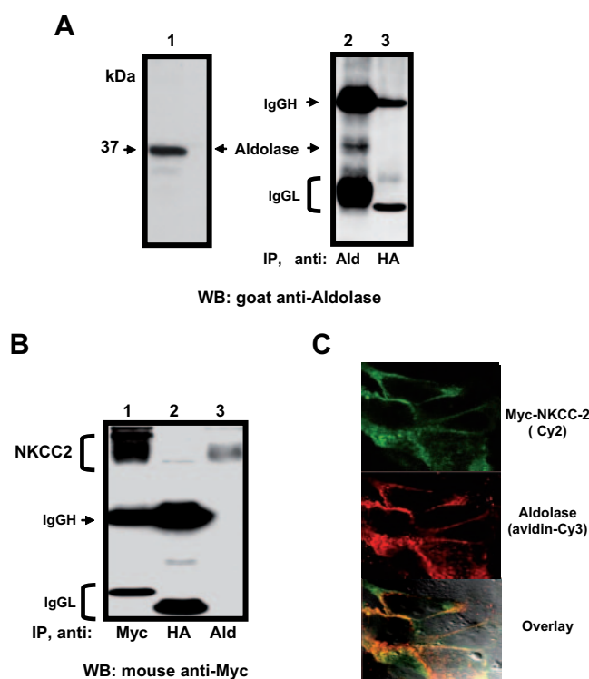
FIGURE 5. NKCC2 co-localizes and interacts with endogenous aldolase protein. A, aldolase endogenous expression in OKP cells. Cell lysates from OKP cells were subjected to immunoprecipitation (IP) using either goat anti-aldolase (Ald) antibody or mouse anti-HA antibody (negative control, upper panel, lane 3). Samples were then reduced (boiled in \beta -mercaptoethanol), evaluated via 7.5–10% SDS-PAGE, and immunoblotted with anti-aldolase antibody. A single protein band around 37 kDa was obtained, corresponding to the expected size band of aldolase B. B, co-immunoprecipitation of aldolase with full-length NKCC2. Cell lysates from OKP cells transiently expressing myc-NKCC2 were immunoprecipitated with anti-Myc antibody (positive control, lower panel, lane 1) or anti-HA (negative control, lower panel, lane 2), or anti-aldolase antibody (lower panel, lane 3). Co-immunoprecipitated NKCC2 with aldolase was detected by immunoblotting using anti-Myc (lower panel, lane 3). IgGH, the heavy chain of immunoglobulin G; IgGL, the light chain of immunoglobulin G. WB, Western blot. C, immunofluorescence staining of aldolase and Myc-NKCC2 proteins. OKP cells were double-stained with anti-Myc and anti-aldolase antibodies. Anti-aldolase and anti-Myc antibodies were visualized with a biotinylated anti-goat IgG antibody and Cy3-labeled streptavidin (red) and Cy2-labeled anti-mouse (green) IgG antibodies, respectively. The yellow color (merged image) indicates co-localization of aldolase and NKCC2 proteins.
