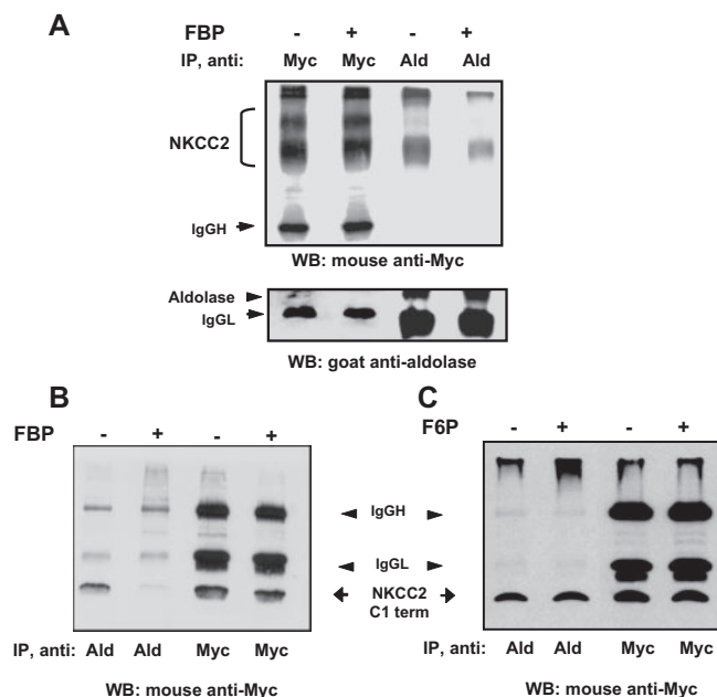
FIGURE 6. Aldolase binding to NKCC2 is specifically inhibited by fructose 1,6-bisphosphate. OKP cells were transfected with NKCC2-Myc (A) or NKCC2-C1-term (B and C). 24 h after transfection, cells were treated overnight with 5 mM FBP or 5 mM fructose 6-phosphate. They were then subjected to immunoprecipitation (IP) using either mouse anti-Myc antibody or goat anti-aldolase (Ald) antibody. The resultant immunoprecipitates were subjected to SDS-PAGE on a 7.5% polyacrylamide gel and then analyzed by immunoblotting using mouse anti-Myc monoclonal antibody or goat anti-aldolase antibody. FBP presence disrupted NKCC2-aldolase interaction (A, upper and lower panels, and B). In contrast to FBP, the structurally similar compound fructose 6-phosphate (F6P) had no effect on the interaction (C) indicating that FBP effect is specific. IgGH, the heavy chain of immunoglobulin G; IgGL, the light chain of immunoglobulin G. WB, Western blot.
