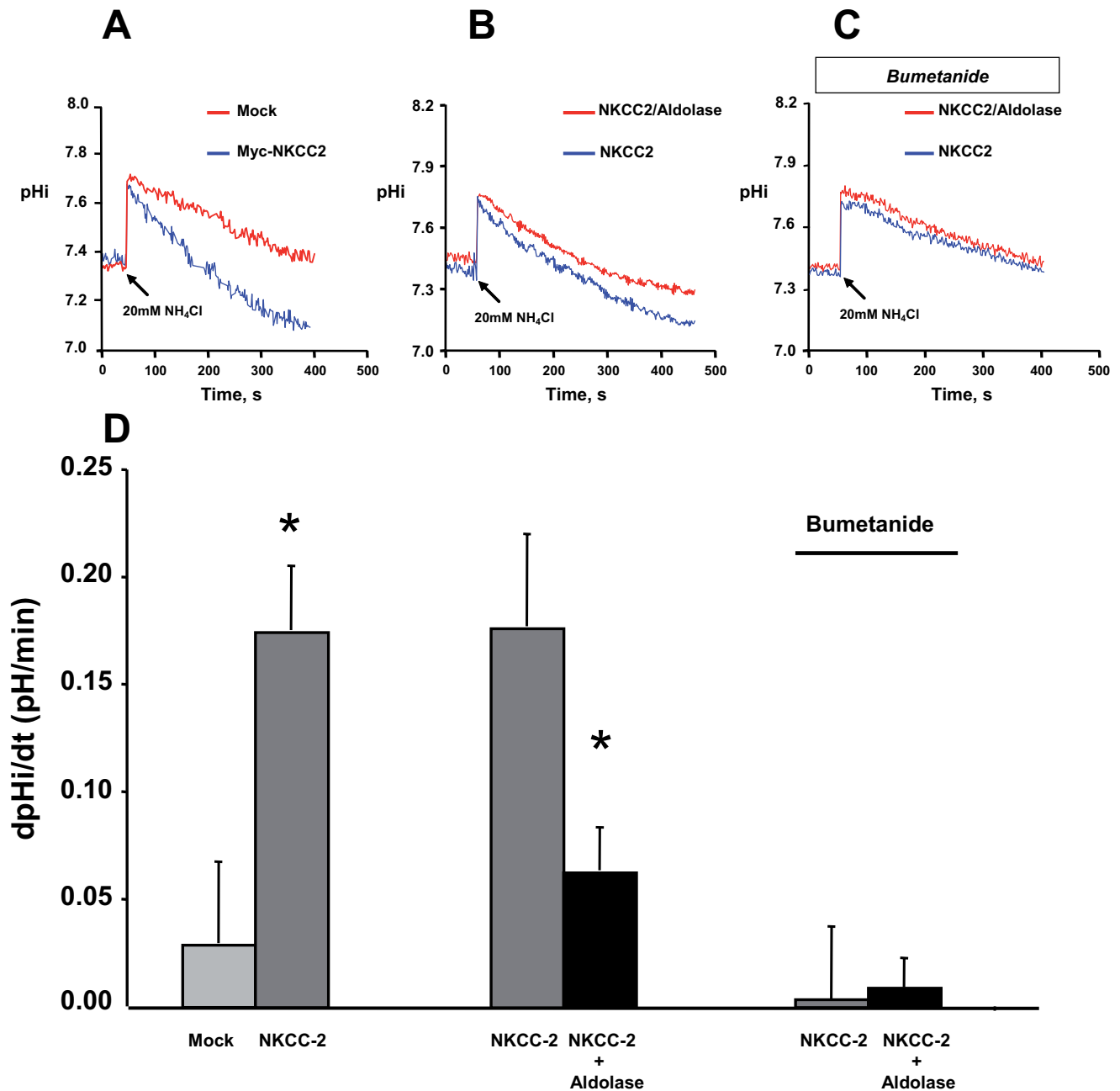
FIGURE 10. Measurement of Na-K(NH 4 + )-Cl co-transport activity in OKP cells expressing Myc-NKCC2. Intracellular pH was measured in confluent monolayers of OKP cells as described under "Experimental Procedures." The arrow indicates replacement with medium containing 20 mM NH 4 Cl (isototically substituted for NaCl). A , Na-K(NH 4 + )-Cl co-transport activity in OKP cells expressing myc-NKCC2 (blue) compared with mock-transfected cells (red). B , effect of aldolase co-expression (red) on NKCC2 activity. C , effect of aldolase co-expression on NKCC2 activity in the presence of 0.1 mM bumetanide. Results of representative experiments are shown. D , mean initial rate of pH i recovery (dpH i /dt) from and NH 4 + -induced alkaline load. Each bar represents the mean ± S.E. rates of cell pH recovery (dpH i /dt, pH units/min) under different experimental conditions (Mock cells, OKP cells expressing Myc-NKCC2, OKP cells co-transfected with NKCC2 and aldolase B, OKP cells co-transfected with NKCC2 and aldolase B in presence 0.1 mM bumetanide). *, p < 0.05.
