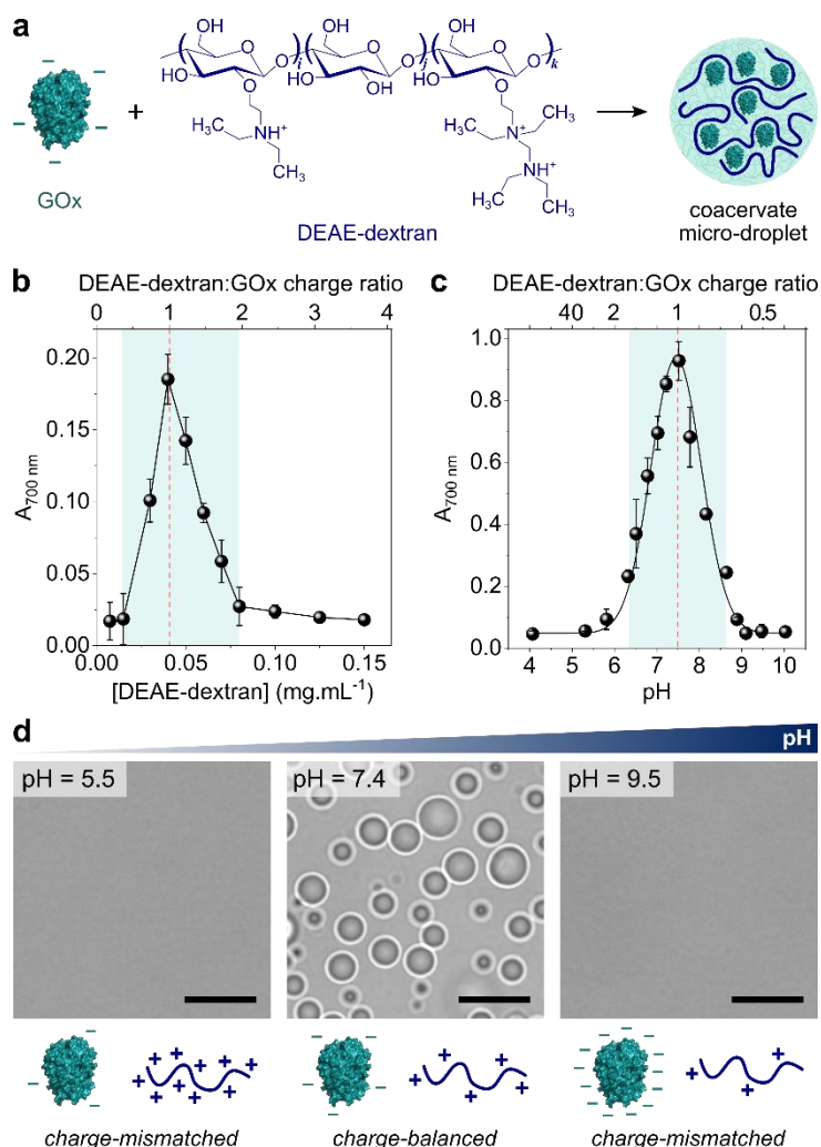
Fig 1 (a) Scheme of the complex coacervation process between glucose oxidase (GOx) and diethylaminoethyl (DEAE)-dextran. (b) Plot of the absorbance at 700 nm of solutions of GOx (0.25 mg mL -1 ) in the presence of varying concentrations of DEAE-dextran in phosphate buffer (2.5 mM, pH 7.4). The maximum turbidity (red dotted line) corresponds to the optimal ratio for coacervation. (c) Plot of the absorbance at 700 nm of a solution of GOx (0.25 mg mL -1 ) and DEAE-dextran (0.04 mg mL -1 ) as a function of the pH. The maximum turbidity (red dotted line) corresponds to the optimal pH for coacervation. On (b) and (c), the DEAE-dextran (positive): GOx (negative) molar charge ratio is also reported (see ESI Note 1†). Error bars represent the standard deviation of three independent repeats. (d) Optical microscopy images of GOx/DEAE-dextran mixtures ([GOx] = 0.25 mg mL -1 , [DEAE-dextran] = 0.04 mg mL -1 ) prepared at different pH, as indicated, and corresponding schematic representations of the charge conditions on both polyions. Scale bars, 10 μm.
