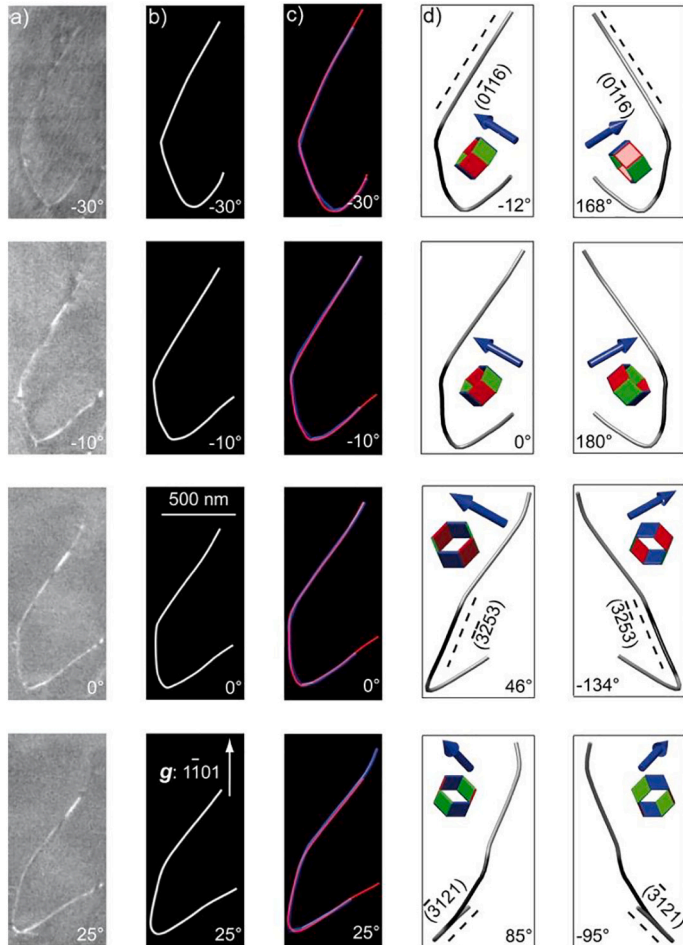
Fig. 4. Reconstruction method for few projected images of Fig. 3 dislocation 1A whose Burgers vector is 1/3[11\bar{2}3] . a) Four aligned projected micrographs (projection angles of -30^\circ , -10^\circ , 0^\circ and 25^\circ ) obtained in WBDF conditions with the \bar{1}101 diffraction vector and a precession angle of 0.1^\circ ; b) corresponding redrawn projected micrographs in black and white contrast; c) superimposed of projected images extracted from the reconstructed volume (in blue) and the redrawn micrographs of Fig. 3b (in red); d) Projected images extracted from the reconstructed volume for eight projected angles, where the (\bar{3}253) plane is edge-on for the projected angles of 46^\circ , the (\bar{3}121) plane is edge-on for the projected angles of 85^\circ and the (0\bar{1}16) plane is edge-on for the projected angles of -12^\circ . This reconstruction gives us the opportunity to characterize three mixed climb systems: \pm 1/3[11\bar{2}3](\bar{3}121) , \pm 1/3[11\bar{2}3](\bar{3}253) and \pm 1/3[11\bar{2}3](0\bar{1}16) (in grey, black and grey respectively), for the same dislocation. The crystal orientation is materialized by the colored hexagonal prism and the Burgers vector is shown by the blue arrow. (For interpretation of the references to colour in this figure legend, the reader is referred to the web version of this article.)
