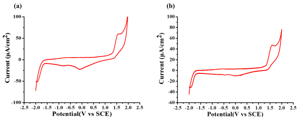
Figure S3. Cyclic voltammetry of electrochemical reactions of dyes 6 and 7 in acetonitrile solvent against saturated calomel electrode (SCE) under nitrogen saturated solution: (a) dye 6; (b) dye 7.
