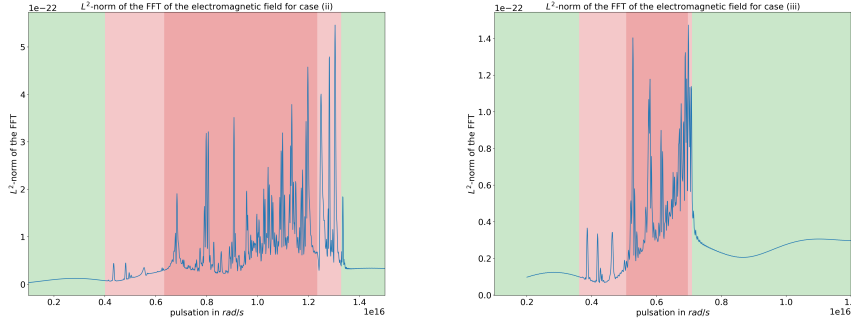
Figure 13: L^2 -norm in space of the time FFT of the whole electromagnetic field for a Gaussian pulse centered at 7 \times 10^{15} \text{rad.s}^{-1} : for case (ii) (left), for case (iii) (right). The green zones indicate when \omega \notin I_\omega , the red zones indicate when \omega \in I_\omega . The darker red zone indicates the critical subinterval \omega \in I_{\omega_b} .
