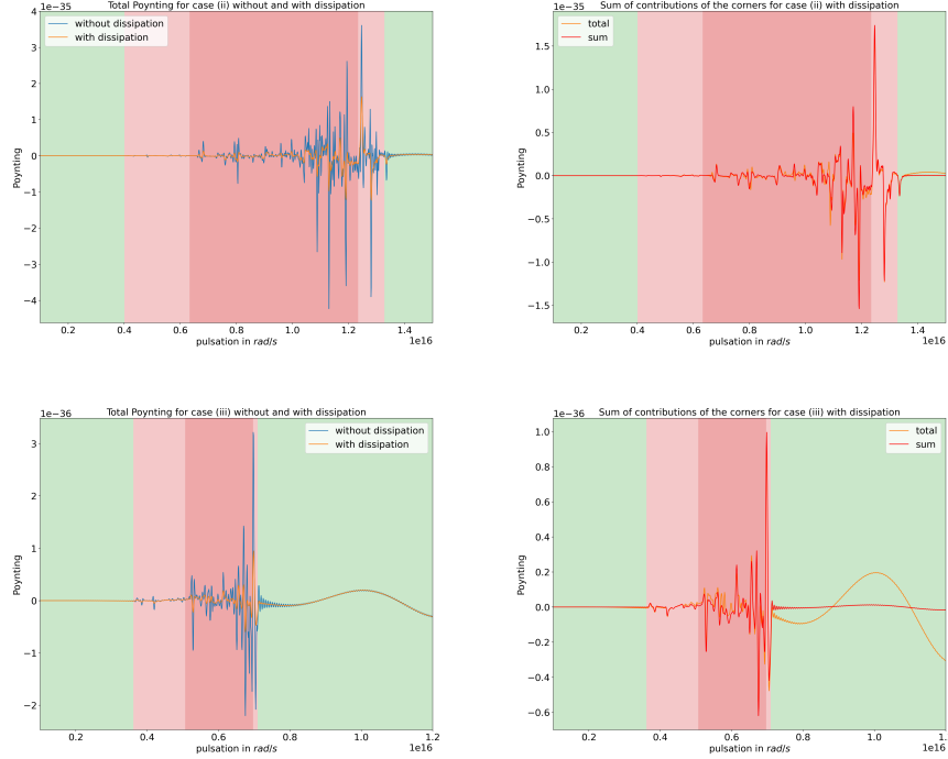
Figure 17: Left: comparison of Poynting fluxes with and without dissipation: case (ii) (top row), case (iii) (bottom row). Right: comparison of total Poynting fluxes and the sum of the Poynting fluxes at the corners: case (ii) with dissipation (top row), case (iii) with dissipation (bottom row).
