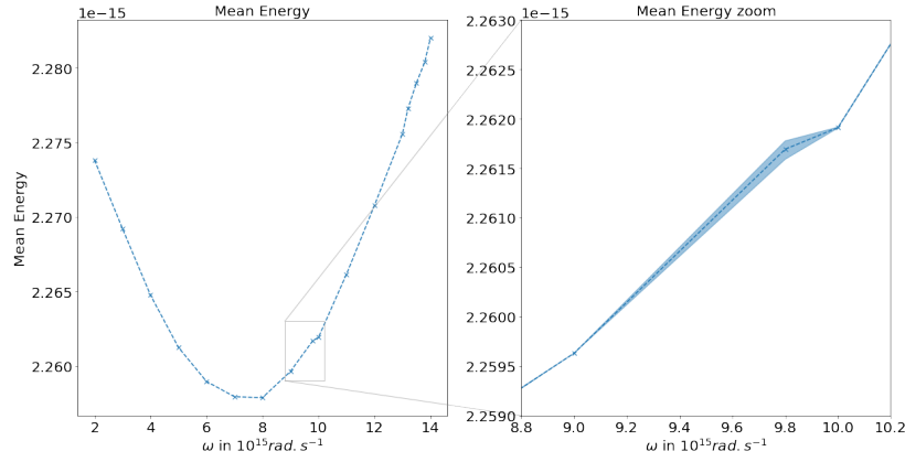
Figure 5: (Left) Mean energy \bar{\mathcal{E}} (computed with (15)) with respect to the incident pulsation. For each value of the pulsation \omega , we compute the mean of the energy on different time intervals of length T(\omega) over the simulation time duration. (Right) Zoom of the energy mean where there is a maximum of variations, scaled by a factor 10. Computations show relative variations of order 10^{-6} .
