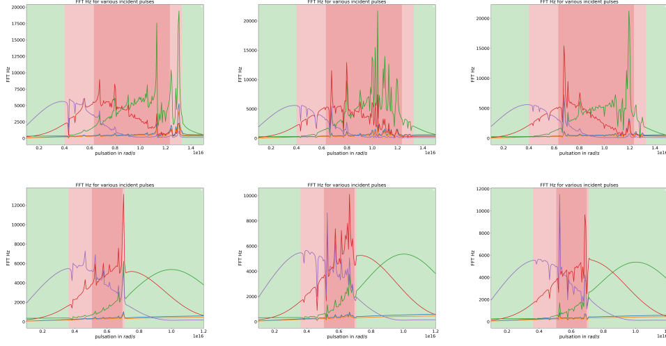
Figure 12: FFT of |H_z| at probe points p_1 (left), p_2 (middle), p_3 (right) for several Gaussian pulses centered at 4 \times 10^{15} , 7 \times 10^{15} or 10 \times 10^{15} \text{rad.s}^{-1} and two widths: for case (ii) (top row), for case (iii) (bottom row). The green zones indicate when \omega \notin I_\omega , the red zones indicate when \omega \in I_\omega . The darker red zone indicates the critical subinterval \omega \in I_{\omega_b} .
