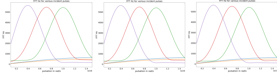
Fig. 7: Modulus of the Fourier transform for various gaussian pulses at probe points p_1 (left), p_2 (middle), p_3 (right) for several Gaussian pulses. We use several central frequencies ( 4 \times 10^{15} , 7 \times 10^{15} and 10 \times 10^{15} \text{rad.s}^{-1} ) and two widths for the pulses.
