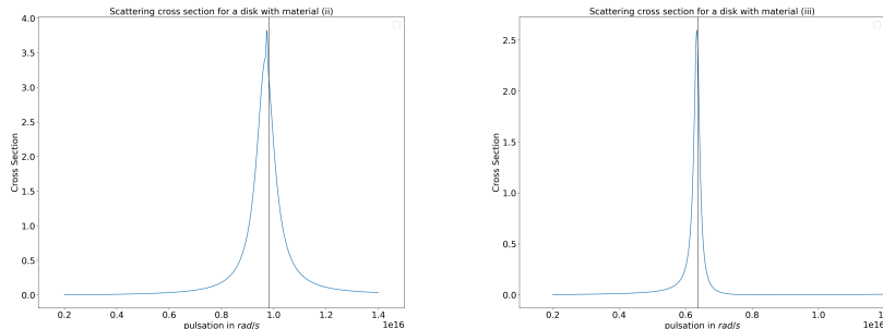
Fig. 18: Scattering cross sections for a disk made of a Drude material (ii) and (iii) (no dissipation). The 2D section of the cylinder (a disk) has the same perimeter as the triangle section used in this work. The maximum is achieved at \omega = 9.74 \times 10^{15} \text{rad.s}^{-1} for case (ii) (0.6% relative error to \omega_{sp} ) and \omega = 6.34 \times 10^{15} \text{rad.s}^{-1} for case (iii) (0.5% relative error to \omega_{sp} ).
