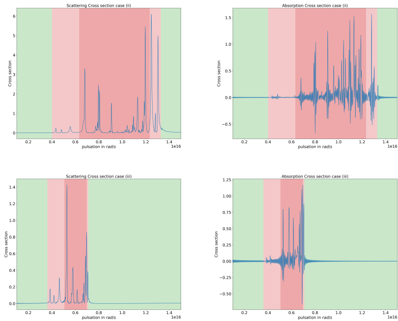
Fig. 14: (Left): Scattering cross sections C_{sca} (computed with (2.18)) when considering a Gaussian pulse: for case (ii) (top row), for case (iii) (bottom row). (Right): Absorption cross sections C_{abs} when considering a Gaussian pulse: for case (ii) (top row), for case (iii) (bottom row).
