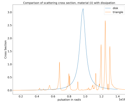
Fig. 19: Comparison of scattering cross sections for a disk made of a Drude material (ii) with dissipation using the triangular section and a disk section with same perimeter as the triangle section.
