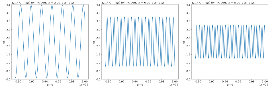
Fig. 4: Representation of \mathcal{E}(t) (computed via (2.6)) for different incident fields. The incident field is monochromatic, we vary the pulsation \omega and represent the result for \omega = 2 \times 10^{15} \text{ rad.s}^{-1} , \omega = 6 \times 10^{15} \text{ rad.s}^{-1} , \omega = 8 \times 10^{15} \text{ rad.s}^{-1} .
