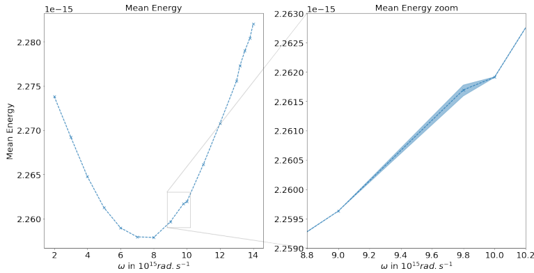
Fig. 5: (Left) Mean energy \underline{\mathcal{E}} (computed with (2.15)) with respect to the incident pulsation. For each value of the pulsation \omega , we compute the mean of the energy on different time intervals of length T(\omega) over the simulation time duration. (Right) Zoom of the energy mean where there is a maximum of variations, scaled by a factor 10. Computations show relative variations of order 10^{-6} .
