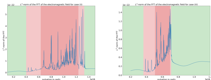
Fig. 13: L^2 -norm in space of the time FFT of the whole electromagnetic field for a Gaussian pulse centered at 7 \times 10^{15} \text{rad.s}^{-1} : for case (ii) (left), for case (iii) (right). The green zones indicate when \omega \notin I_\omega , the red zones indicate when \omega \in I_\omega . The darker red zone indicates the critical subinterval \omega \in I_{\omega_b} .
