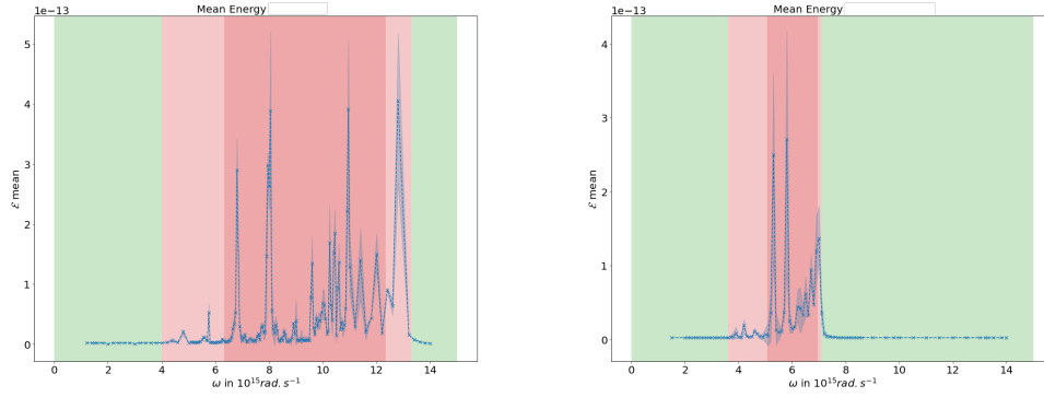
Fig. 9: Mean of energy \underline{\mathcal{E}} (computed with (2.15)) with respect to the monochromatic pulsation: for case (ii) (left), for case (iii) (right). The green zones indicate when \omega \notin I_\omega , the red zones indicate when \omega \in I_\omega . The darker red zone indicates the critical subinterval \omega \in I_{\omega_b} .
