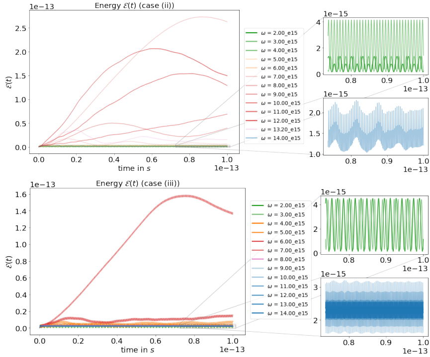
Fig. 8: Representation of \mathcal{E}(t) (computed via (2.6)) for different incident fields for case (ii) (top) and for case (iii) (bottom), with zooms at the long time simulation. The green and blue curves correspond to \omega \notin I_\omega , whereas the warm colored curves correspond to \omega \in I_\omega .
