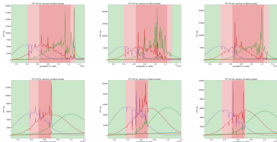
Fig. 12: FFT of |H_z| at probe points p_1 (left), p_2 (middle), p_3 (right) for several Gaussian pulses centered at 4 \times 10^{15} , 7 \times 10^{15} or 10 \times 10^{15} \text{rad.s}^{-1} and two widths: for case (ii) (top row), for case (iii) (bottom row). The green zones indicate when \omega \notin I_\omega , the red zones indicate when \omega \in I_\omega . The darker red zone indicates the critical subinterval \omega \in I_{\omega_b} .
