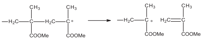
Scheme 2. Depropagation for unzipping.
