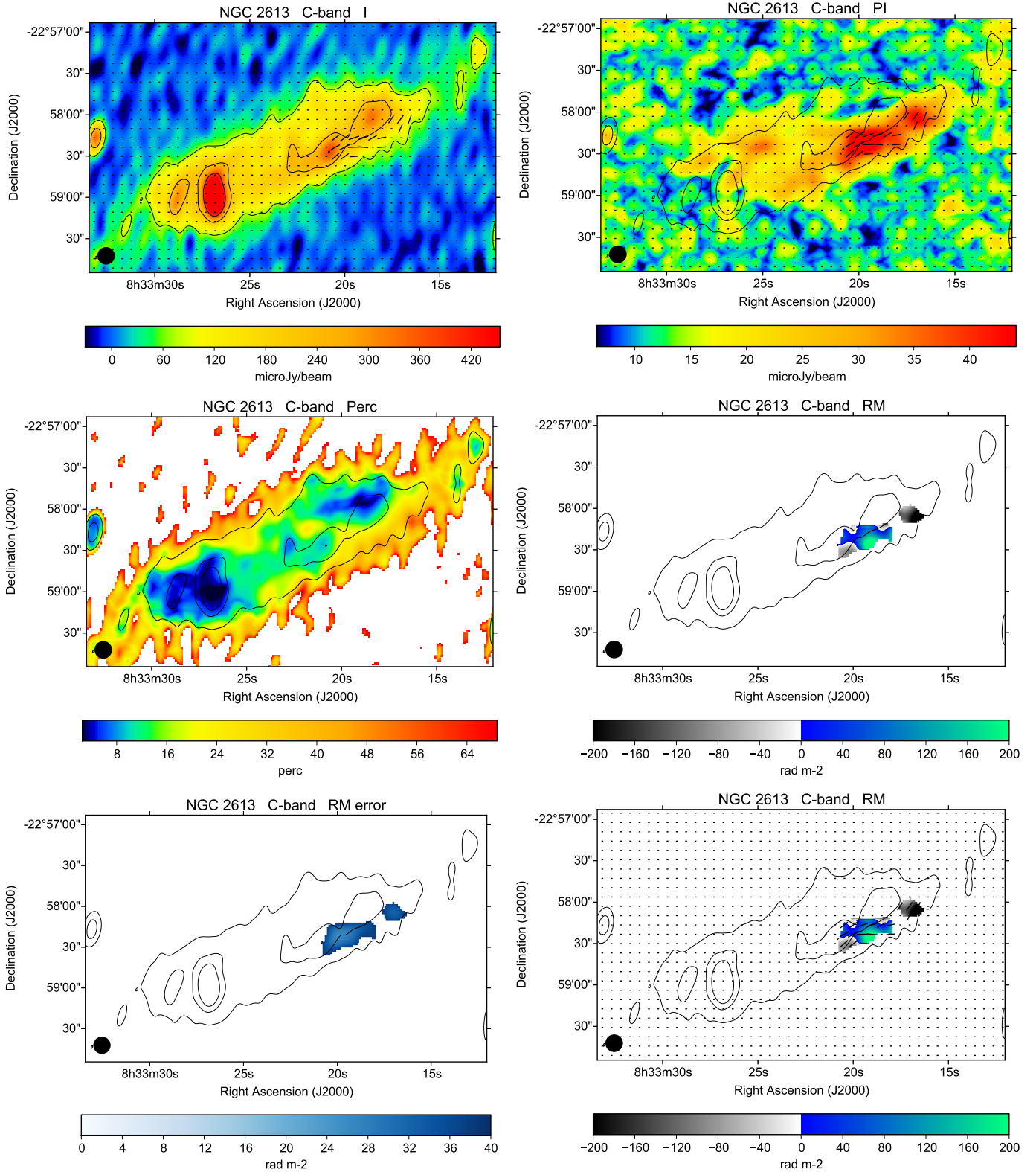
Fig. A.3. Polarization results for NGC 2613 at C-band and 12'' HPBW, corresponding to 1360 pc. The contour levels (TP) are 75, 225, and 375 \mu\text{Jy beam}^{-1} .
