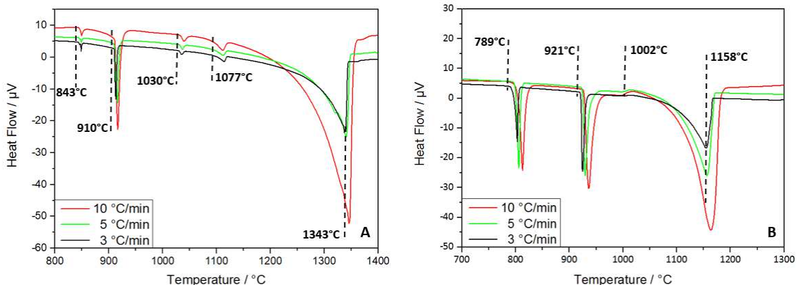
Figure 5 : DTA curves of samples: A) CuFeSi-1; and B) CuFeSi-2. Results obtained at heating rates of 3, 5 and 10 ^{\circ}\text{C}/\text{min} are shown. Transitions are measured at, respectively, 843, 910, 1030, 1077 and 1343 ^{\circ}\text{C} , and 789, 921, 1002 and 1158 ^{\circ}\text{C} . All the transitions are very well reproducible.
