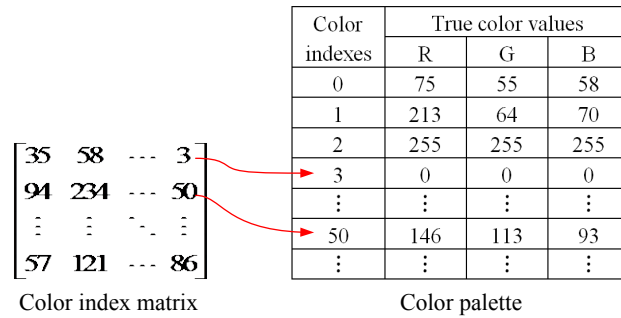
Figure 3: Demonstration of the palette format
