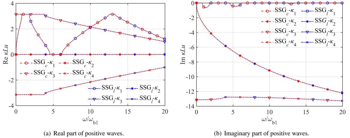
Figure 12: Dispersion relation for periodic Euler-Bernoulli beam by SSG (subscript c of SSG means continuum model, l is lattice model).
