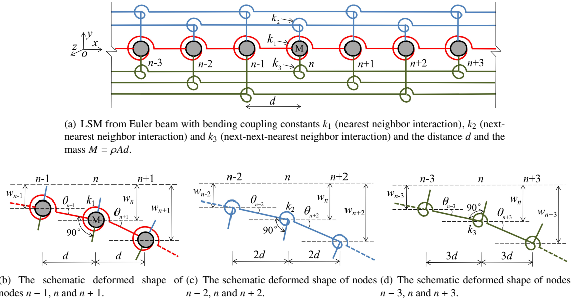
Figure 3: Sketch of a LSM beam.
