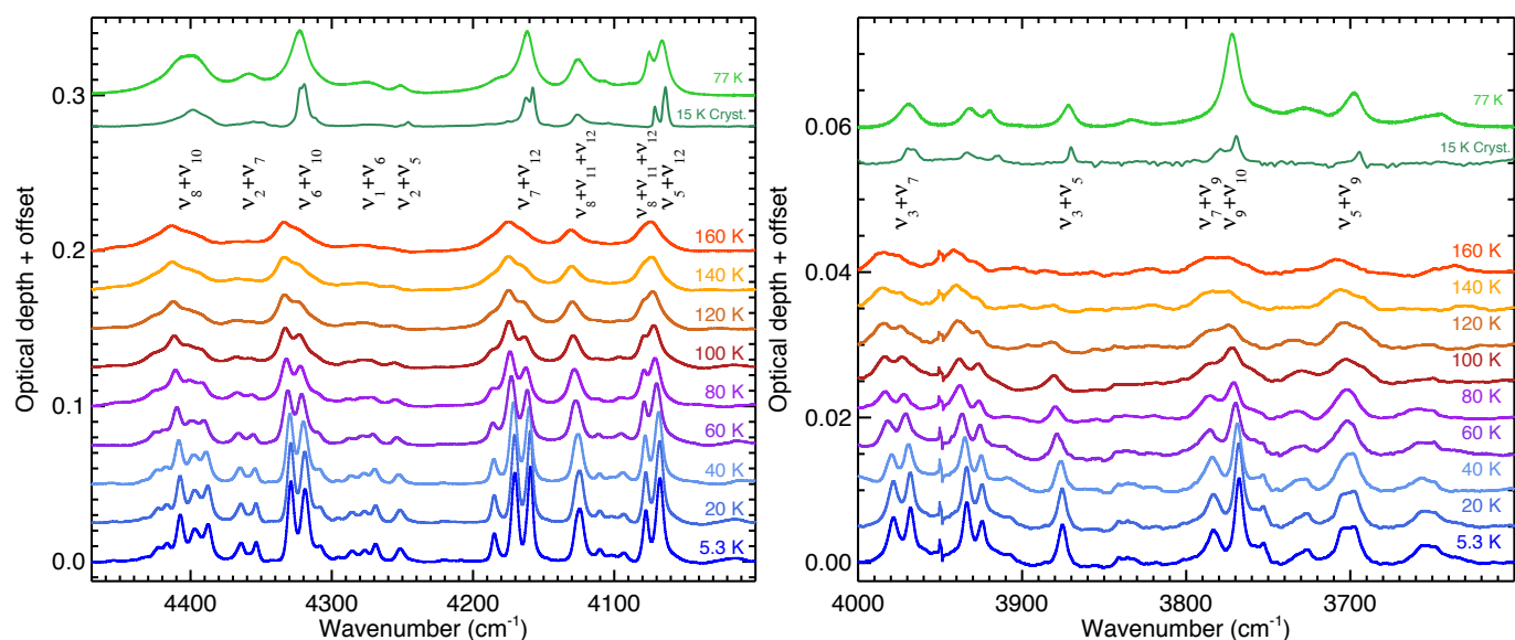
Fig. 3. Temperature dependent infrared spectra of the ethane clathrate in the combination/overtone regions. The crystalline pure ethane spectrum of Hudson et al. (2014) recorded at 15K is shown above. The pure ethane spectrum recorded in the cell at 77K is shown above too. Tentative assignments of the implied vibrational modes are given (see text for details). Spectra are offset for clarity.
