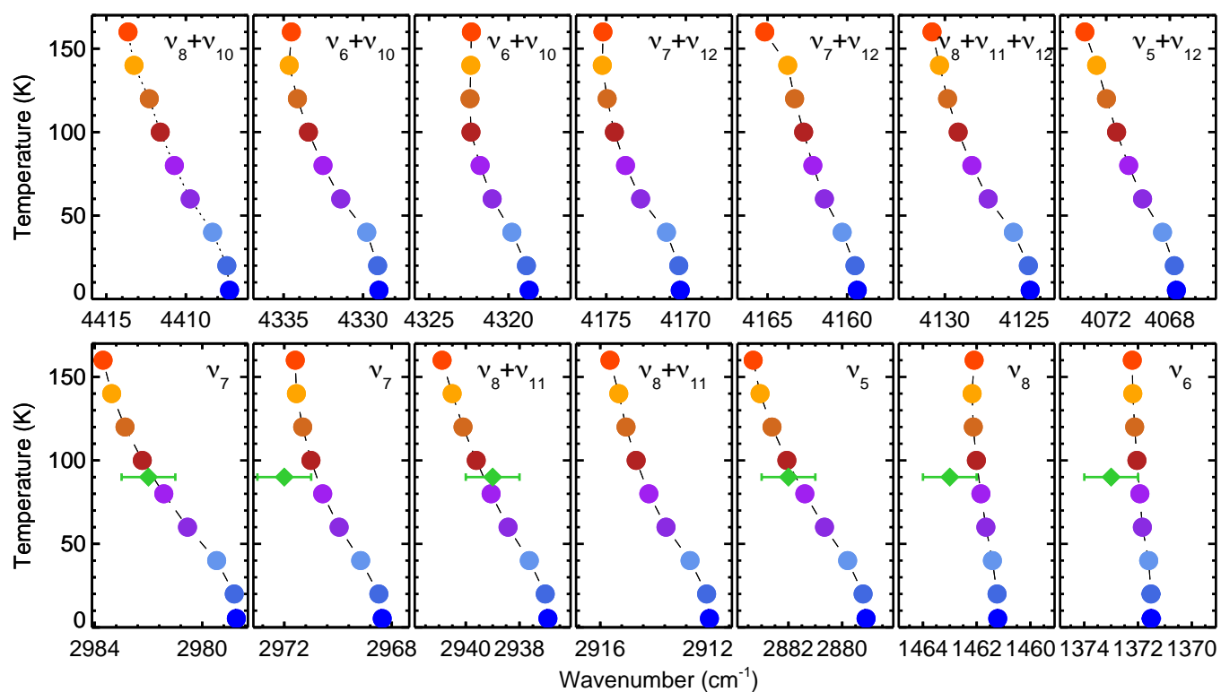
Fig. 4. Temperature dependent positions for selected transitions (circles), with their tentative vibrational assignments, given in Table 1. The ethane centroid vibrational positions for an ethane:oxirane (7:3) mixed clathrate spectrum from Richardson et al. (1985) recorded at 90K, are shown with green diamonds. Oxirane is known to form and induce a clathrate hydrate type I structure, helping to confirm the structure formed and also assign the C_2H_6 vibrational bands in this mixed oxirane clathrate hydrate.
