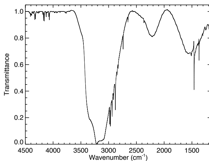
Fig. 1. Baseline corrected ethane clathrate hydrate transmittance spectrum recorded at 5.3K. Note the imperfect cancellation of the Fabry-Perot fringes in the space between the ZnSe windows, leading to small waves observed superimposed on the spectrum (e.g. in the 2500-1700 \text{cm}^{-1} interval). Scattering effects deform the water ice bands because of imperfect film surface roughness once clathration is achieved.
