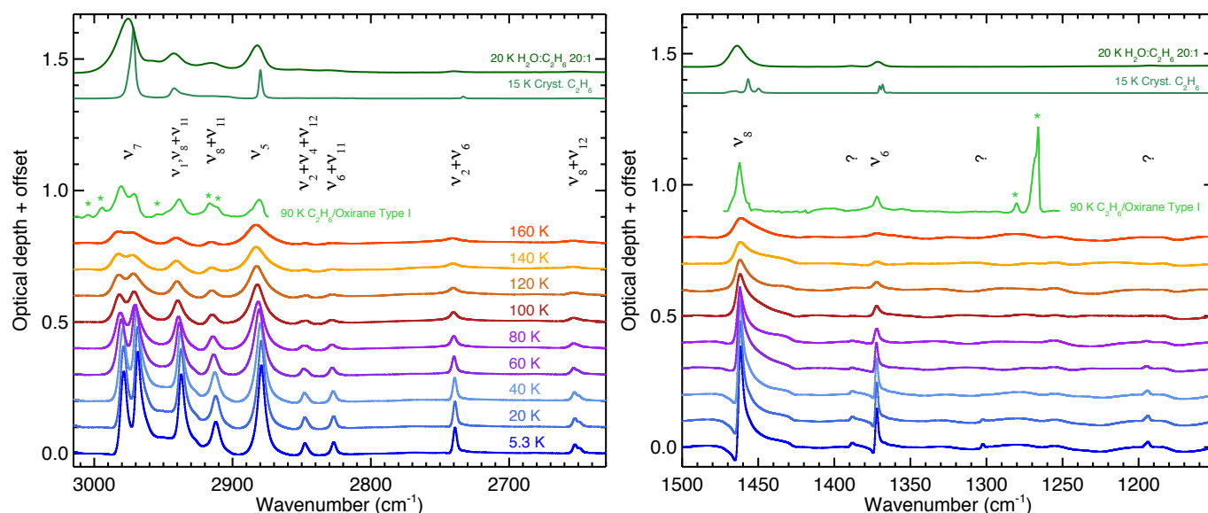
Fig. 2. Temperature-dependent infrared spectra of the ethane clathrate in the fundamental modes regions. The crystalline pure ethane spectrum of Hudson et al. (2014) recorded at 15K is shown above. The infrared spectrum of an \text{H}_2\text{O}:\text{C}_2\text{H}_6 (20:1) ice mixture from the Cosmic Ice Laboratory (Hudson et al., https://science.gsfc.nasa.gov/691/cosmicice/spectra.html ), recorded at 20K, is shown above. The ethane:oxirane (7:3) mixed clathrate spectrum from Richardson et al. (1985) recorded at 90K is also shown. It is baseline corrected, and oxirane features are labelled with asterisks for clarity. Tentative assignments of the implied vibrational modes are given (see text for details). Spectra are offset for clarity.
