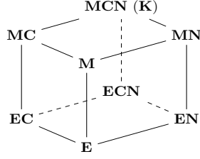
Figure 2: The classical cube.
