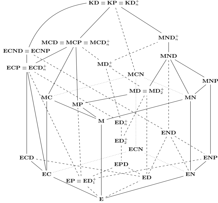
Figure 3: Diagram of deontic systems (“Pantheon”).
