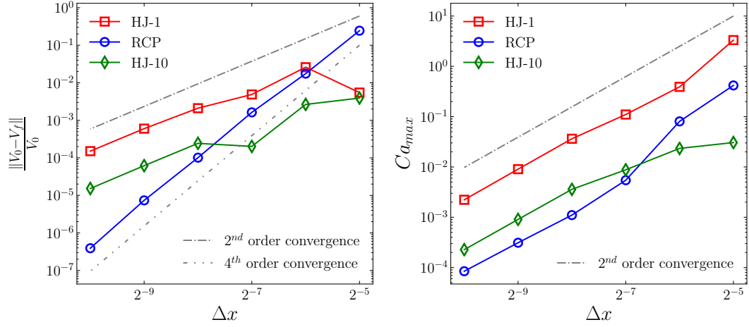
Figure 16: 2D column at equilibrium test case: convergence study for the enclosed volume variation (left) and Ca_{max} (right) at La = 120 for HJ-1, HJ-10 and RCP when a steady state has been reached.
