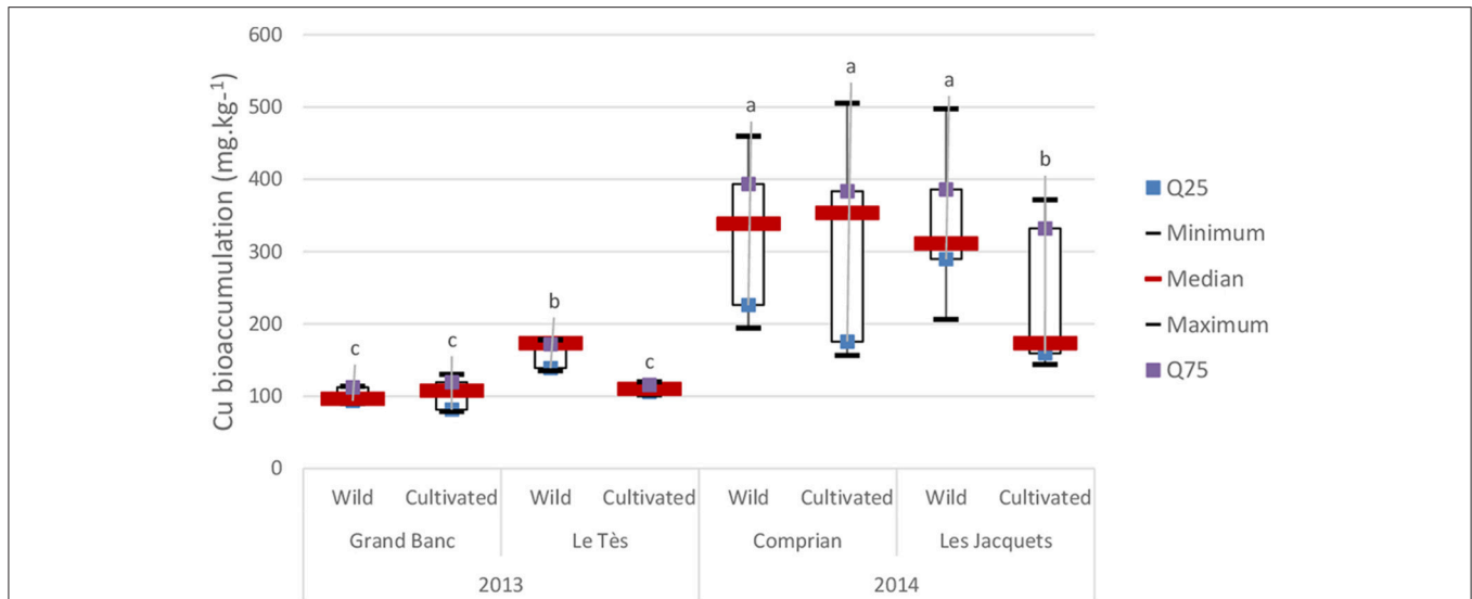
FIGURE 2 | Copper bioaccumulation ( \text{mg Kg}^{-1} ) in adult oysters from different locations in the Arcachon Bay. Box plots represent the minimum, maximum, median, 1st quartile (Q25), and 3rd quartile (Q75) concentrations for 30 individuals per condition in 2013 and 50 individuals in 2014. Data are expressed in \text{mg Kg}^{-1} dry weight \pm SD.
