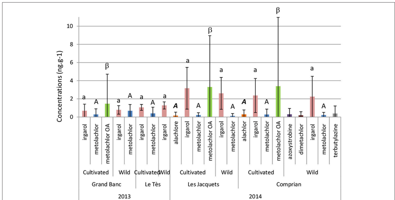
FIGURE 3 | Pesticide bioaccumulation ( \text{ng g}^{-1} ) in summer 2013 and 2014 in adult oysters. Data represent the average concentrations in \text{ng g}^{-1} dry weight \pm SD of the 3 sampling dates in 2013 and the 5 sampling dates in 2014. Each sample represents a pool of 10 oysters. Statistical analysis was performed on each individual pesticide.
