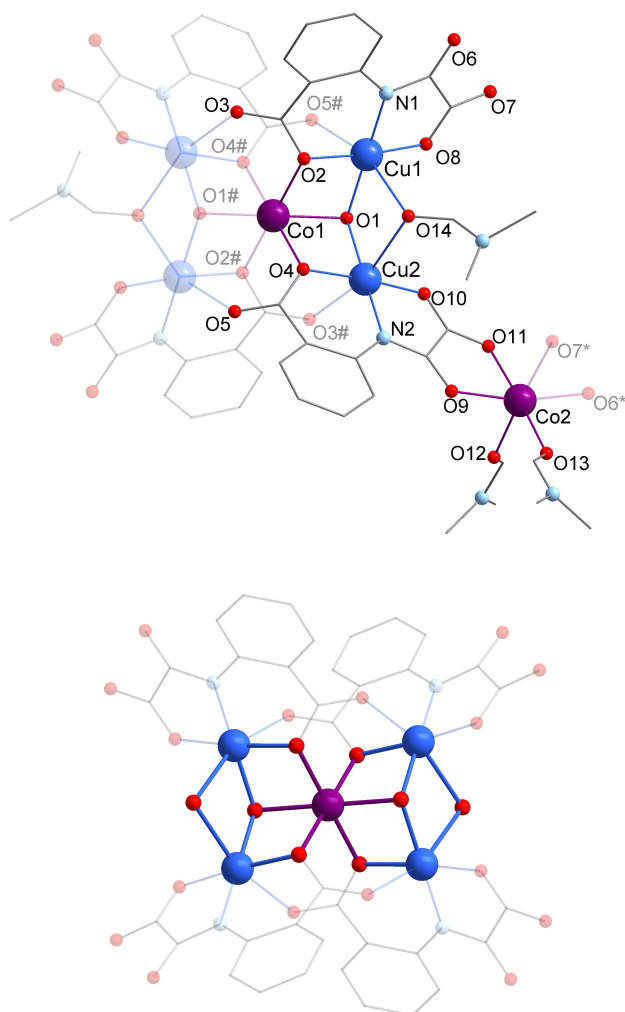
Figure 2. (top) View of the asymmetric unit in the crystal structure of compound 1 . (symmetry codes: #: 1-x,2-y,1-z; *: 1-x,1-y,1-z). (bottom) representation of the lacunar bis-cubane pentametalllic core. H atoms and non-coordinated solvent molecules have been omitted for clarity.
