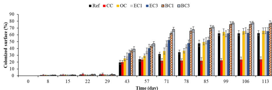
Figure 17. Quantification of marine fowler organisms using an image-analysis-based method. Ref = control concrete; CC = cured concrete; OC = oiled concrete; EC1 = ECOPODE™ concrete prepared with CEM I; EC3 = ECOPODE™ concrete prepared with CEM III; BC1 = biomimetic concrete prepared with CEM I; BC3 = biomimetic concrete prepared with CEM III. Each experiment was performed on 15 replicates, and the error bars present the standard deviation of the values obtained.
