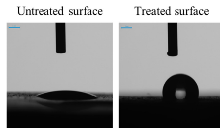
Figure 15. Contact angle of a water drop on the surface of untreated mortar and mortar treated with a curing compound. Photos were taken two seconds after contact between the water and the surface.
