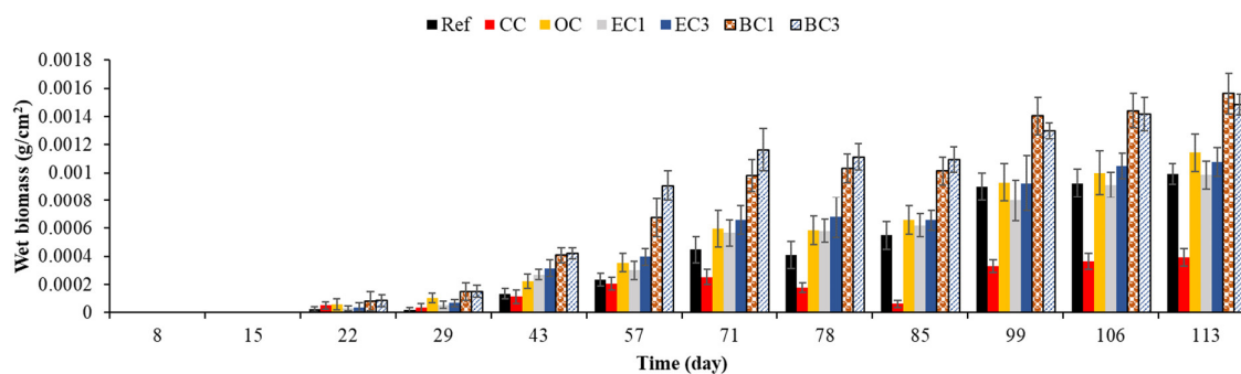
Figure 18. Quantification of marine fouler organisms using wet-weight biomass measurement. Ref = control concrete. CC = cured concrete; OC = oiled concrete; EC1 = ECOPODE™ concrete prepared with CEM I; EC3 = ECOPODE™ concrete prepared with CEM III; BC1 = biomimetic concrete prepared with CEM I; BC3 = biomimetic concrete prepared with CEM III. Each experiment was performed on 15 replicates, and the error bars present the standard deviation of the values obtained.
