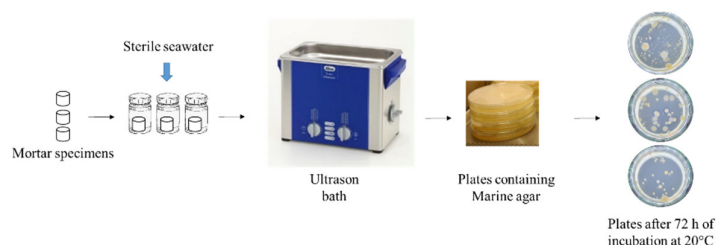
Figure 6. Culture-based method used in the quantification of bacterial biofilm formed on the surface of mortar specimens.
