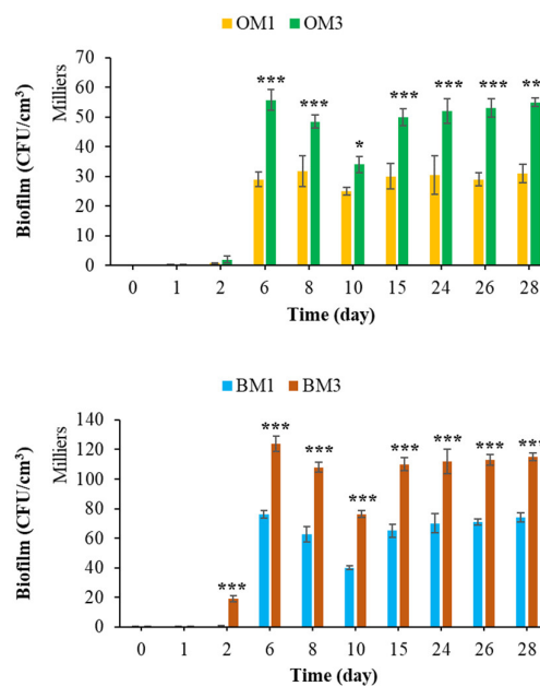
Figure 13. Quantification of bacterial biofilm on CEM1 and CEM3 mortar specimens. Each experiment was performed in triplicate, and the error bars present the standard deviation of the values obtained. Ref = control mortar; OM1 = oiled mortar prepared with CEM I; OM3 = oiled mortar prepared with CEM III; BM1 = biomimetic mortar prepared with CEM I; BM3 = biomimetic mortar prepared with CEM III. The experiments highlighted with asterisks differed significantly from the control (Bonferroni; *, p < 0.05 , ***, p < 0.001 ) at the indicated time.
