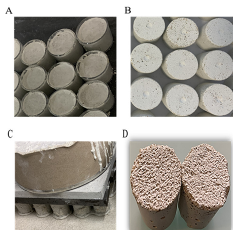
Figure 2. Preparation of mortar specimens. (A) Preparation of SS mortar specimens (mortars in molds); (B) SS mortar specimens obtained after stripping; (C) preparation of RS mortar specimens on rough silicone skin; (D) RS mortar specimens obtained after stripping.
