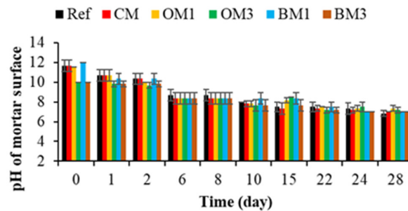
Figure 10. Evaluation of the pH of mortar surfaces. Each evaluation was performed in triplicate, and the error bars present the standard deviation from the values obtained. Ref = control mortar; CM = cured mortar; OM1 = oiled mortar prepared with CEM I; OM3 = oiled mortar prepared with CEM III; BM1 = biomimetic mortar prepared with CEM I; BM3 = biomimetic mortar prepared with CEM III.
