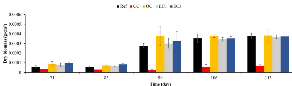
Figure 19. Quantification of marine fouler organisms using dry-weight biomass measurement. Ref = control concrete; CC = cured concrete; OC = oiled concrete; EC1 = ECOPODE™ concrete prepared with CEM I; EC3 = ECOPODE™ concrete prepared with CEM III. Each experiment was performed in triplicate, and the error bars present the standard deviation of the values obtained.
