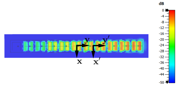
Fig. 8. Surface currents normalized amplitude of the 11-patch array (value averaged over one phase cycle): measurement coordinate system (x, y) (geometric center) and optimized one (x', y') .
