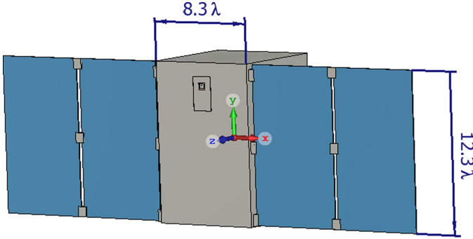
Fig. 10. Simulated model of the antenna (a patch) on a platform satellite (a simplified version of ANGELS) with the patch antenna at 11 GHz and the measurement coordinate system.
