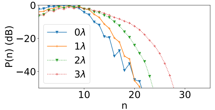
Fig. 5. Normalized n -spectra of the horn antenna at 30 GHz for different translations over the z -axis.
