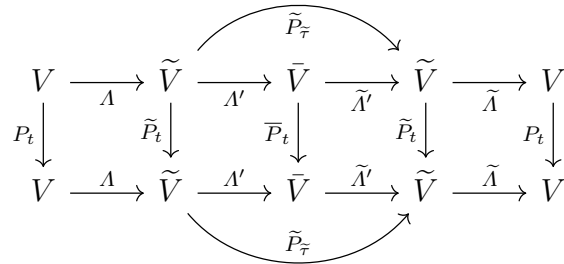
Figure 2: Transitive interweaving relations
