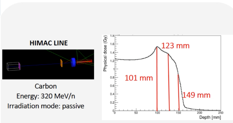
HSG cells irradiated at 3 positions of the SOBP, in 2002. Kagawa et al. (2002)
