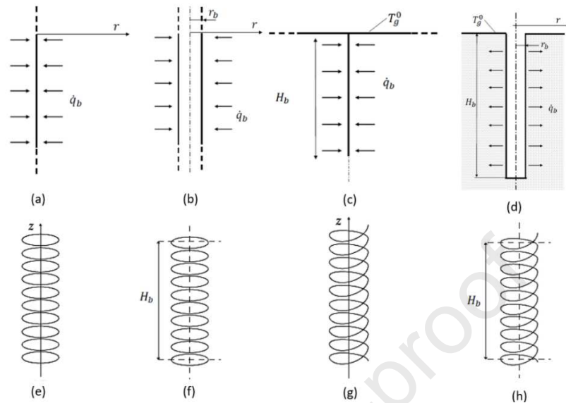
Figure 3. Schematic representation of the main analytical models for vertical GHE analysis: (a) ILSM, (b) ICSM, (c) FLSM, (d) SCSM, (e) IRSM, (f) FRSM, (g) ISSM, (h) FSSM
