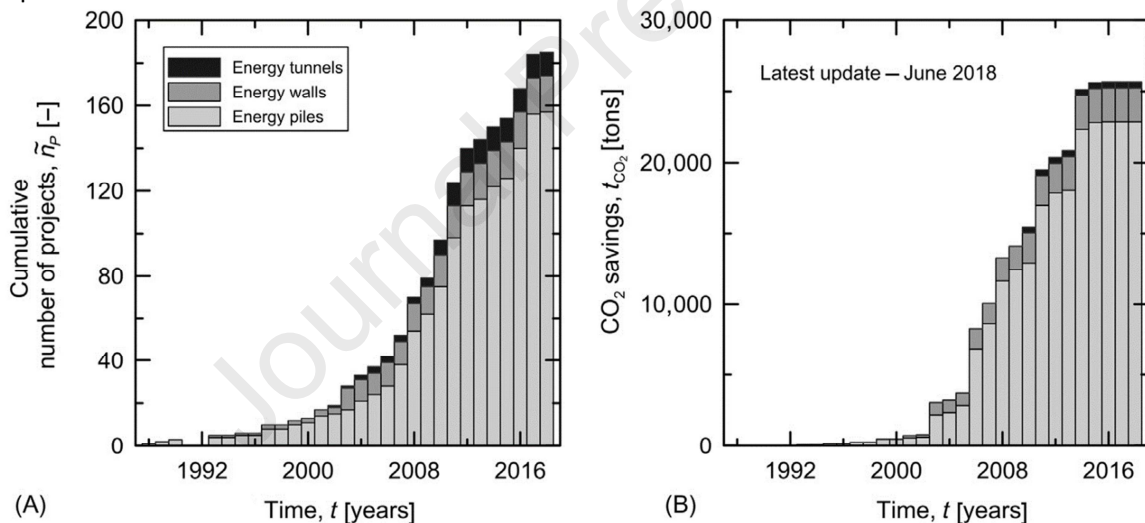
Figure 1. Cumulative number of (A) energy geostructure projects worldwide and (B) carbon dioxide savings worldwide [16].
