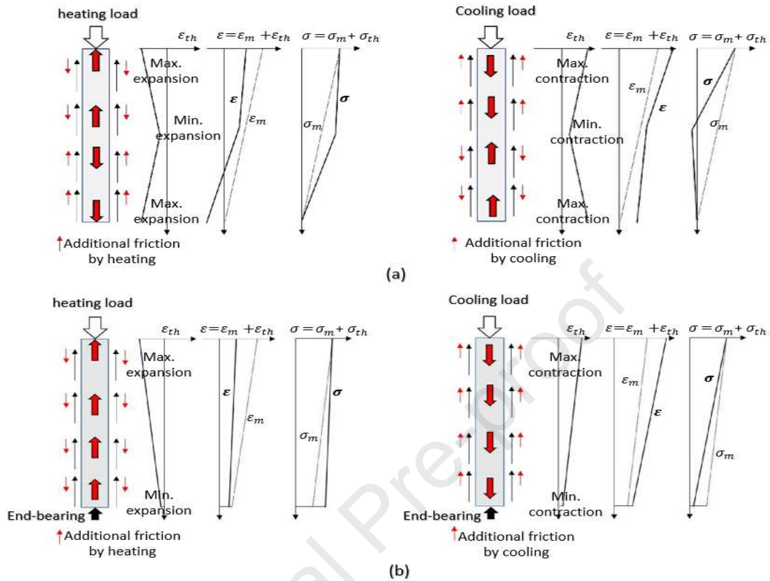
Figure 4. Thermo-mechanical performance of (a) friction pile and (b) end-bearing pile [60].
