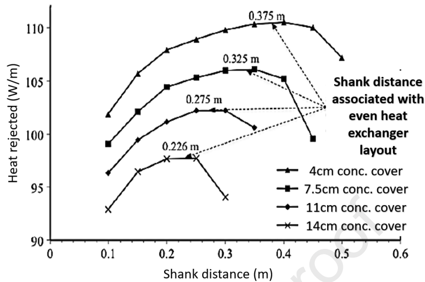
Figure 9. The effect of the shank distance and the concrete cover on the thermal performance of energy piles [47]
