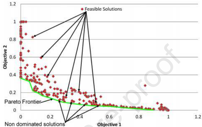
Figure 11. An example of Pareto Front for two-objective functions [134]
