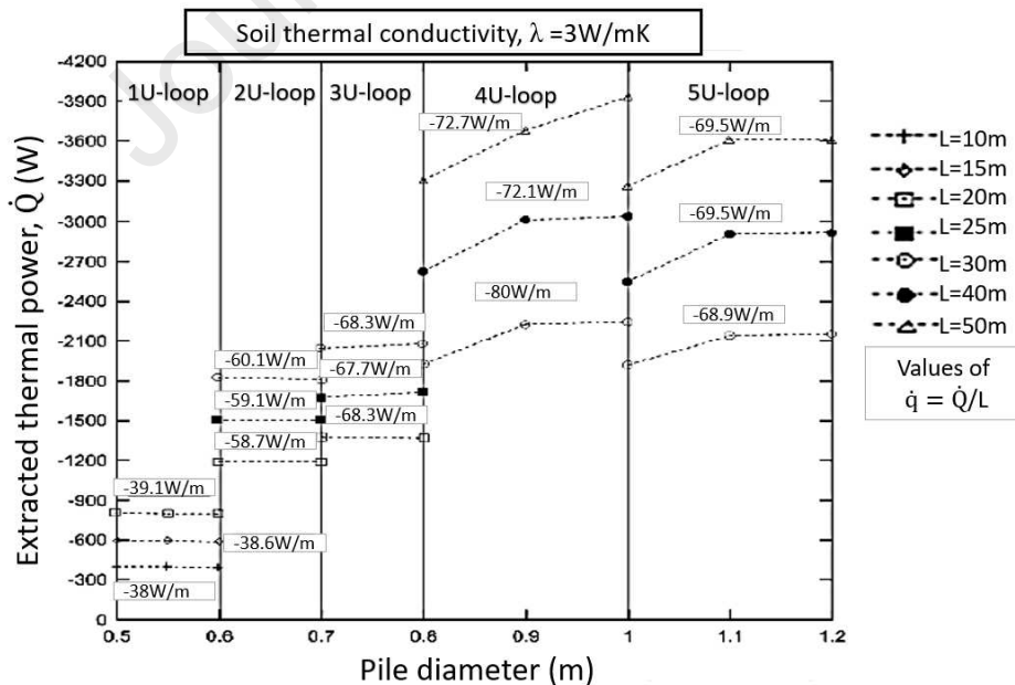
Figure 6. The effect of the diameter and length of the energy piles on their thermal performance [16]
