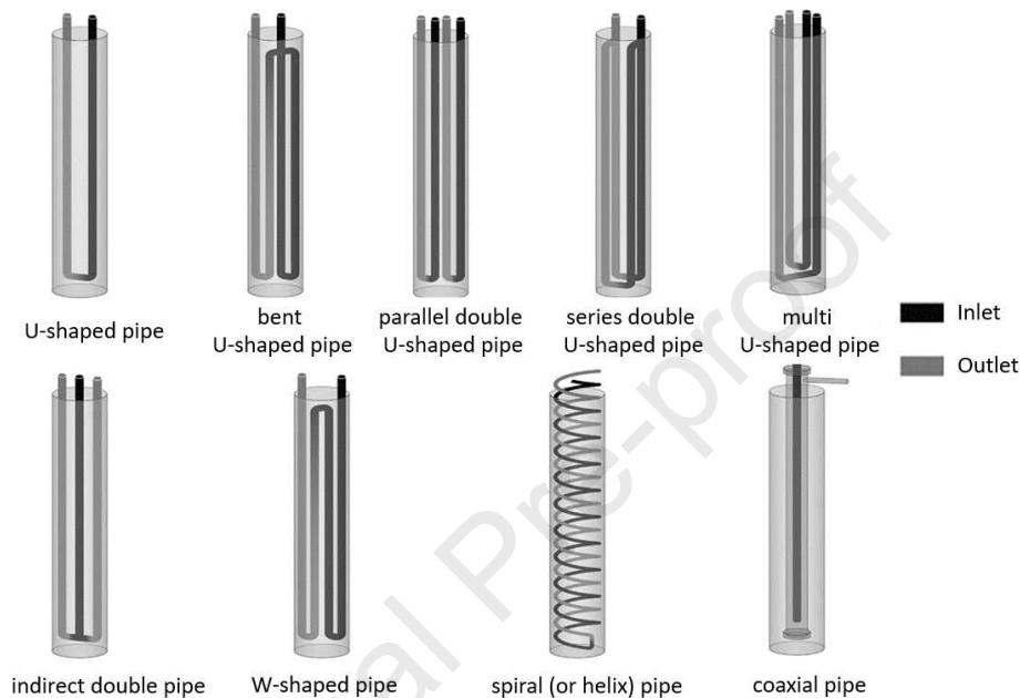
Figure 7. Pipe configurations for energy piles [16]
