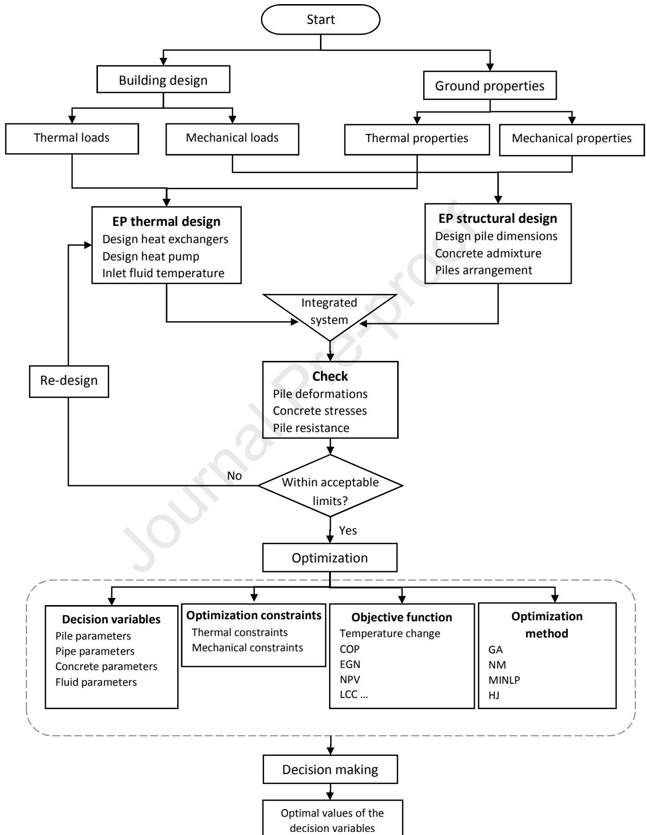
Figure 12. The developed optimization approach for energy piles design
