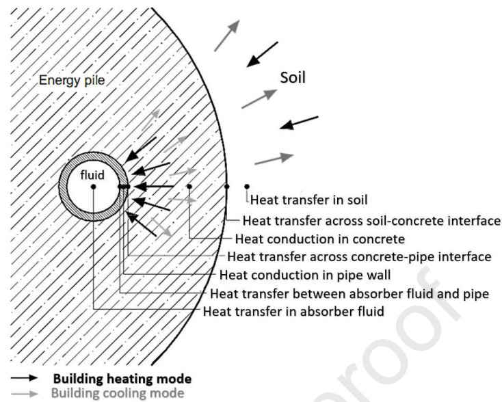
Figure 2. Heat transfer stages in an energy pile
