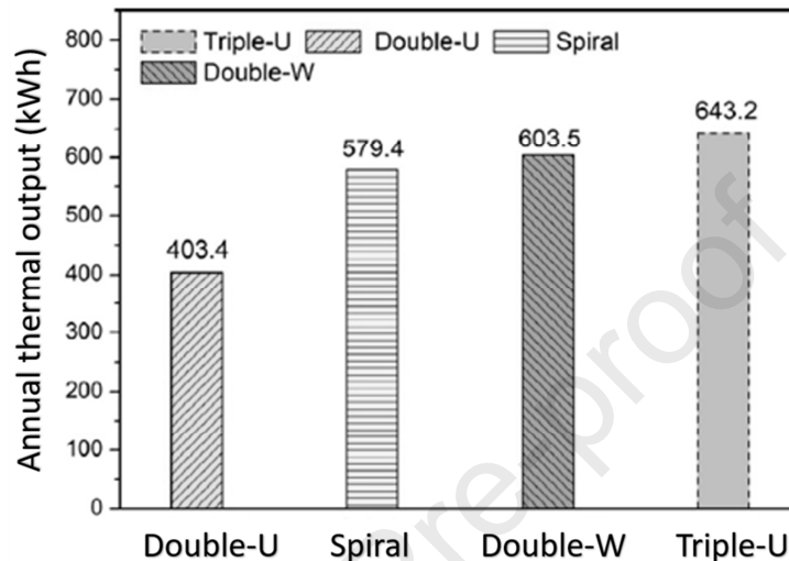
Figure 8. The effect of the pipe configuration on the thermal performance of energy piles [86]
