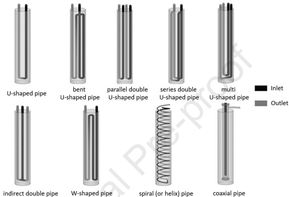
Figure 7. Pipe configurations for energy piles [16]
