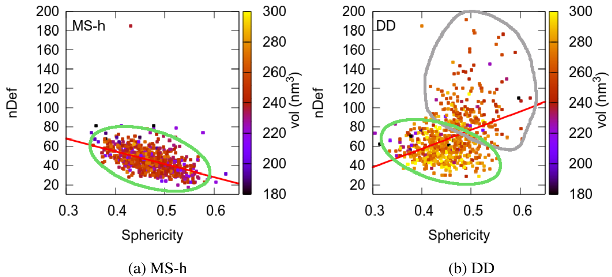
Figure 7: correlation plots between the number of defects (nDef) and the sphericity for MS-h (a) and DD (b). The red lines correspond to simple linear regression between the two variables. For DD, two clusters of points are visible; the points which are within the grey lines correspond to atypical cascades and are responsible for the positive correlation with a simple
