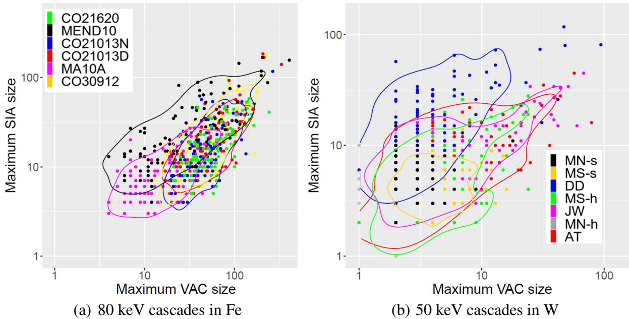
Figure 4: Maximum SIA cluster size vs maximum vacancy cluster size for all the potentials. Each point corresponds to one cascade, the solid curves are the 95% isocontour of the kernel density estimation, which estimates the region containing 95% of the cascade and the highest density of points. The points which lie outside the solid lines are cascades with extreme values.
