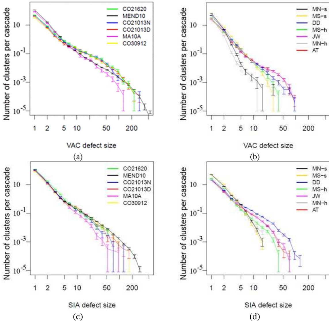
Figure 3: point defect cluster size distributions in 80 keV displacement cascades created in Fe (a) and (c) and 50 keV displacement cascades created in W (b) and (d). (a) and (b): vacancy cluster, (c) and (d): SIA cluster. The bin width increases exponentially and each data point corresponds to the sum of all the clusters having a size within the bin, divided by the bin width and the number of cascades. The vertical bars correspond to the standard error.
