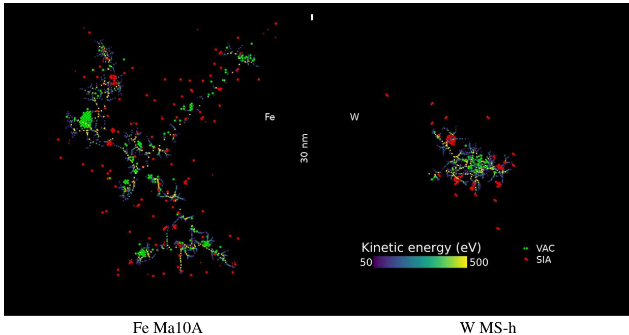
Figure 8: typical cascade morphologies: red spheres represent the SIAs, green spheres represent vacancies. For these pictures, 30 frames have been selected between 0 and 0.2 ps. The cubes represent positions where one atom, in any of the frames, has a kinetic energy higher than 40 eV in Fe and 80 eV in W. The 30 frames are superimposed here, so as to underline the trajectories of atoms of energy large enough to create one vacancy.
