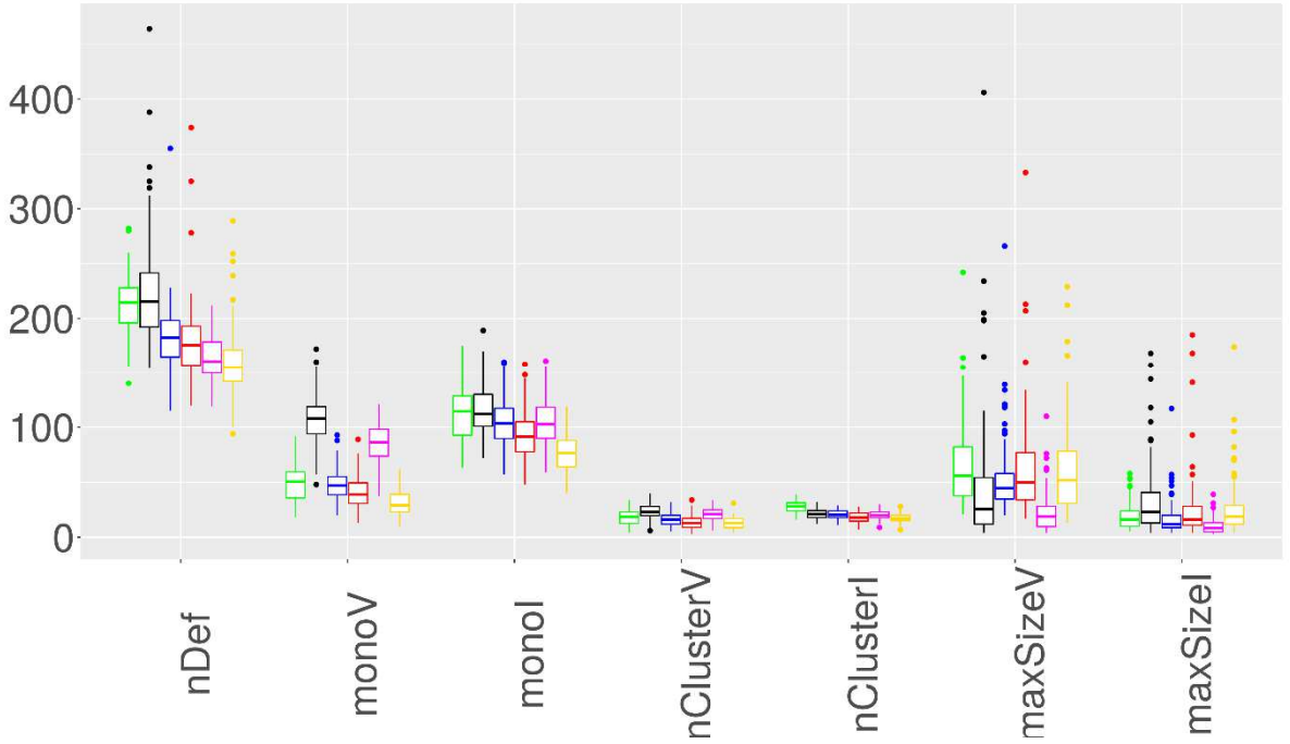
(a) Fe
