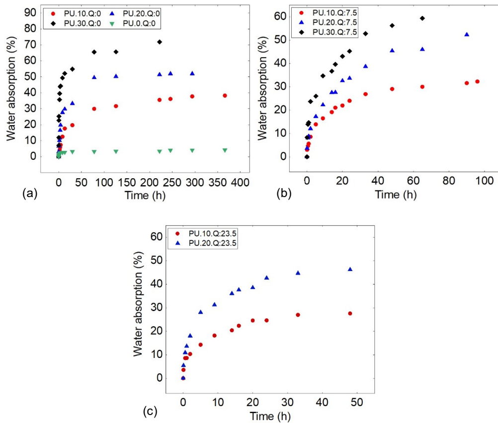
Figure 3. Water absorption percentage in accordance to the time of the incubation for different percentages of the drug at (a) static state, (b) the flow rate of 7.5 ml/s, and (c) 23.5 ml/s. (In PU.x.Q:y: x is indicator of drug percentage and y is indicator of flow rate (ml/s))
