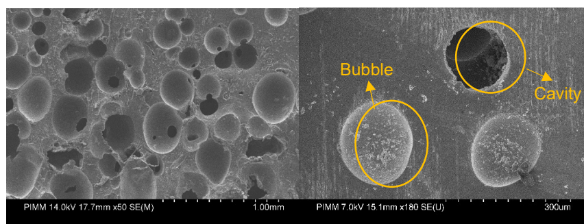
Figure 11. Microscopic images representing the size of hole (PU.10. Q:7.5 after 1 hour the test)
