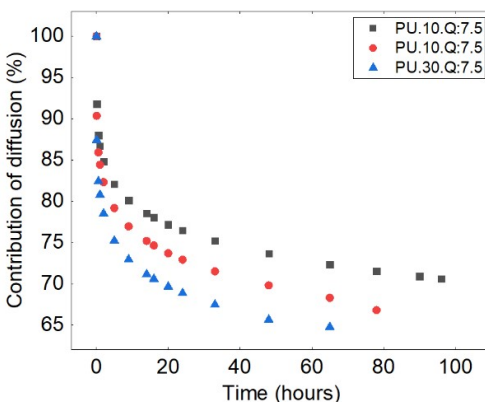
Figure 12. Contribution of diffusion in accordance with the time of the release at different initial drug percentages at the Q=7.5 ml/s
