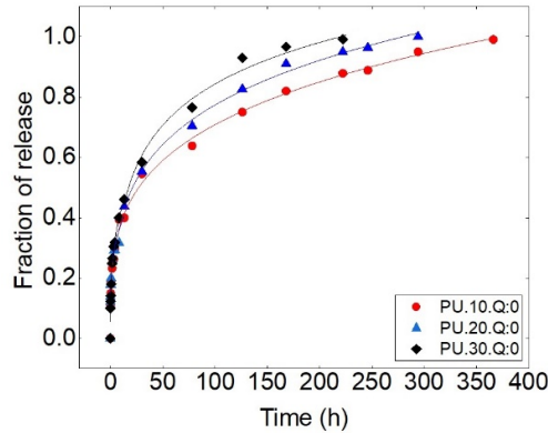
Figure 8. Regression results of PU.10.Q:0, PU.20.Q:0 and PU.30.Q:0 in two steps with Korsmeyer- Peppas model
