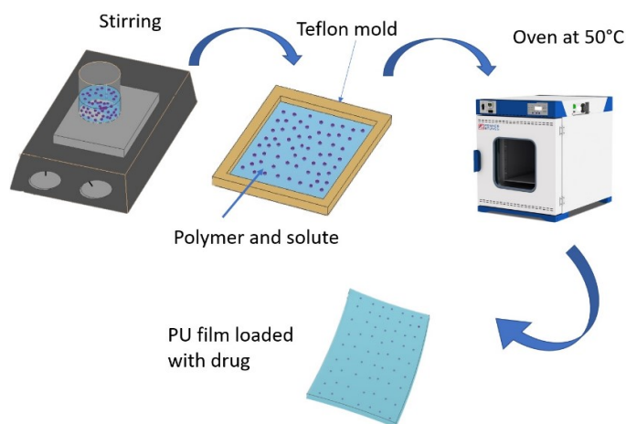
Figure 1. Process of casting for preparing PU films with the diclofenac dispersed inside
