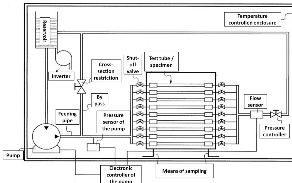
Figure 2. Equipment elements for tests at different flow rates
