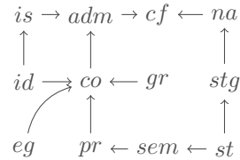
FIGURE 2 – Extension Inclusion Graph Inc(\mathcal{S})
