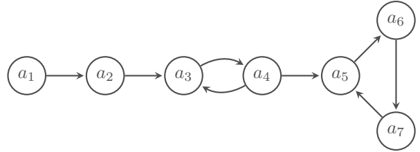
FIGURE 1 – The AF F_1
