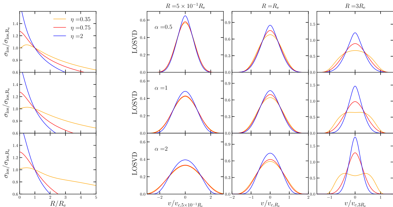
Figure 5. Kinematic observables in one-component models. Orange, red, and blue curves are for models with \eta = 0.35 , 0.75 , and 2 , respectively. Panels in the left column show line-of-sight velocity dispersions, normalized to \sigma_{\text{los},R_e} \equiv \sigma_{\text{los}}(R_e) , when \alpha = 0.5, 1 , and 2 . The other three panels show LOSVDs with the velocity scale normalized to v_{c,R} , the circular speed at the radius of observation R , which increases from left to right: R = 5 \times 10^{-1} R_e , R = R_e , and R = 3R_e . The value of \alpha increases from top to bottom: \alpha = 0.5, 1 , and 2 .
