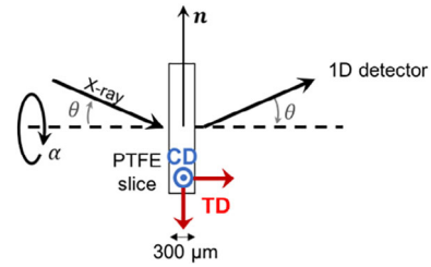
FIGURE 3 Sketch of the \theta - \theta diffraction setup. The sample is rotated along the horizontal axis to record the diffracted intensity along \alpha . The normal n is rotating in the PTFE slice from the compaction direction (CD) for \alpha = 0^\circ to the transverse direction (TD) for \alpha = 90^\circ [Color figure can be viewed at wileyonlinelibrary.com ]
