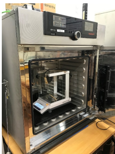
Fig. 1: Instruments setup.
