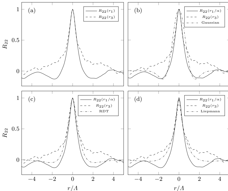
FIGURE 9. Vertical velocity correlation coefficient calculated on a plane at x_2^+ = 165 in the streamwise ( r_1 ) and transverse ( r_3 ) directions. Ratio of streamwise to transverse length scales: \alpha = 1.35 .
