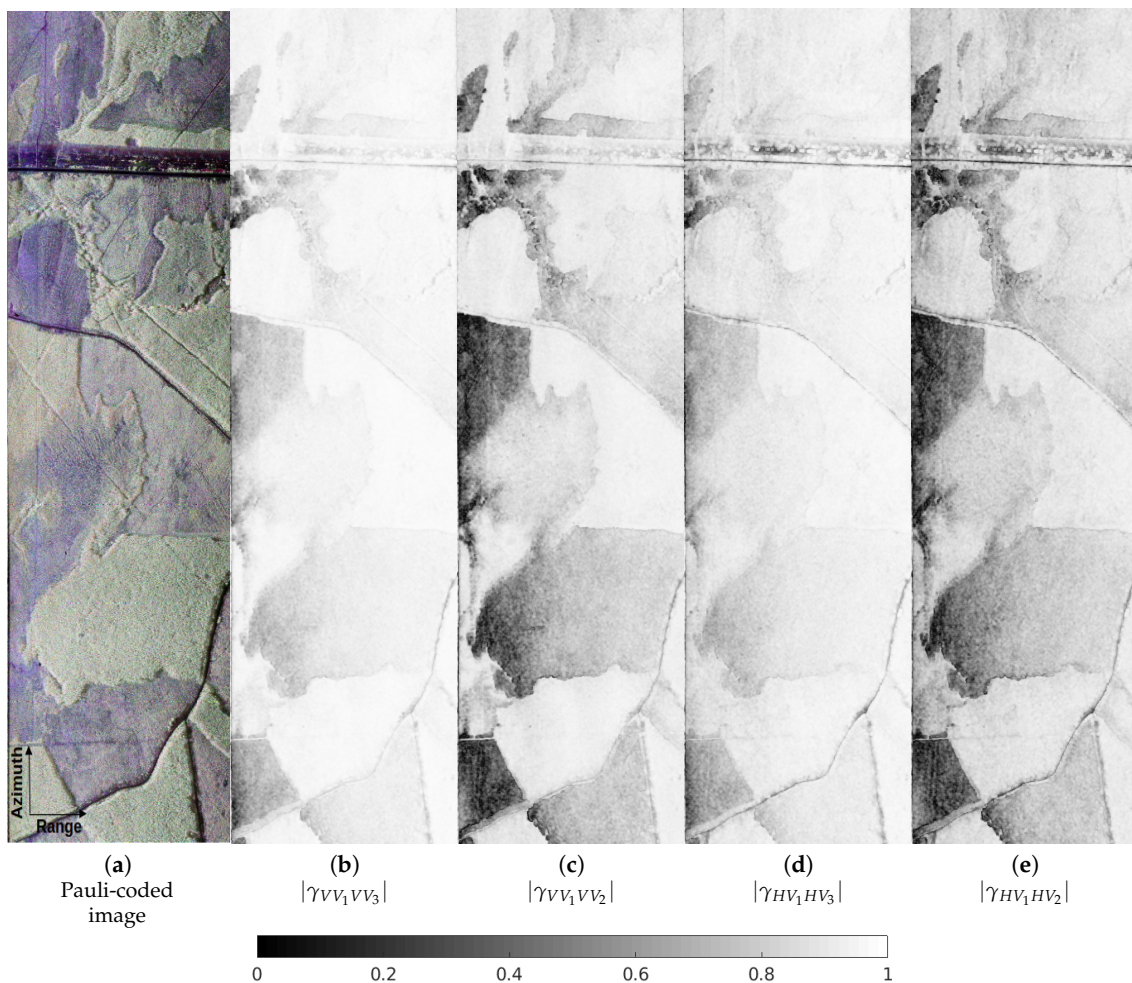
Figure 5. InSAR coherences over the test site.
