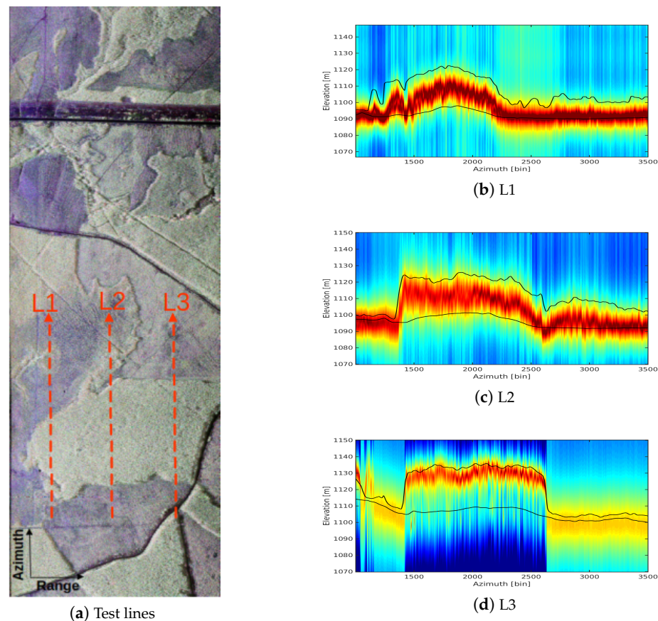
Figure 8. P-MUSIC tomograms for test lines located in near, mid and far range, respectively. n_s = 2 . The black line is the LiDAR ground and tree top elevation estimates.
