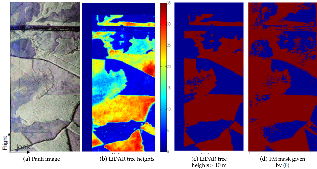
Figure 15. Generated forest/non-forest mask.
