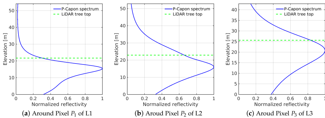
Figure 7. Normalized vertical reflectivity profiles estimated by P-Capon technique at the locations indicated in Figure 6. Elevation here is measured with respect to the LiDAR ground elevation.
