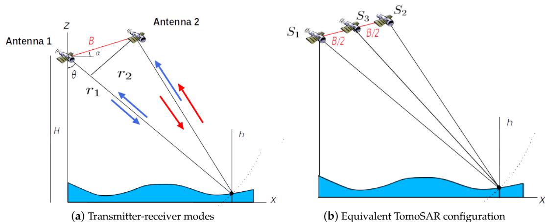
Figure 3. Illustration of transmit–receive modes and equivalent dual-baseline TomoSAR configuration. S_1 and S_2 are the real positions of Antenna 1 and Antenna 2, whereas S_3 is the virtual resulting position.
