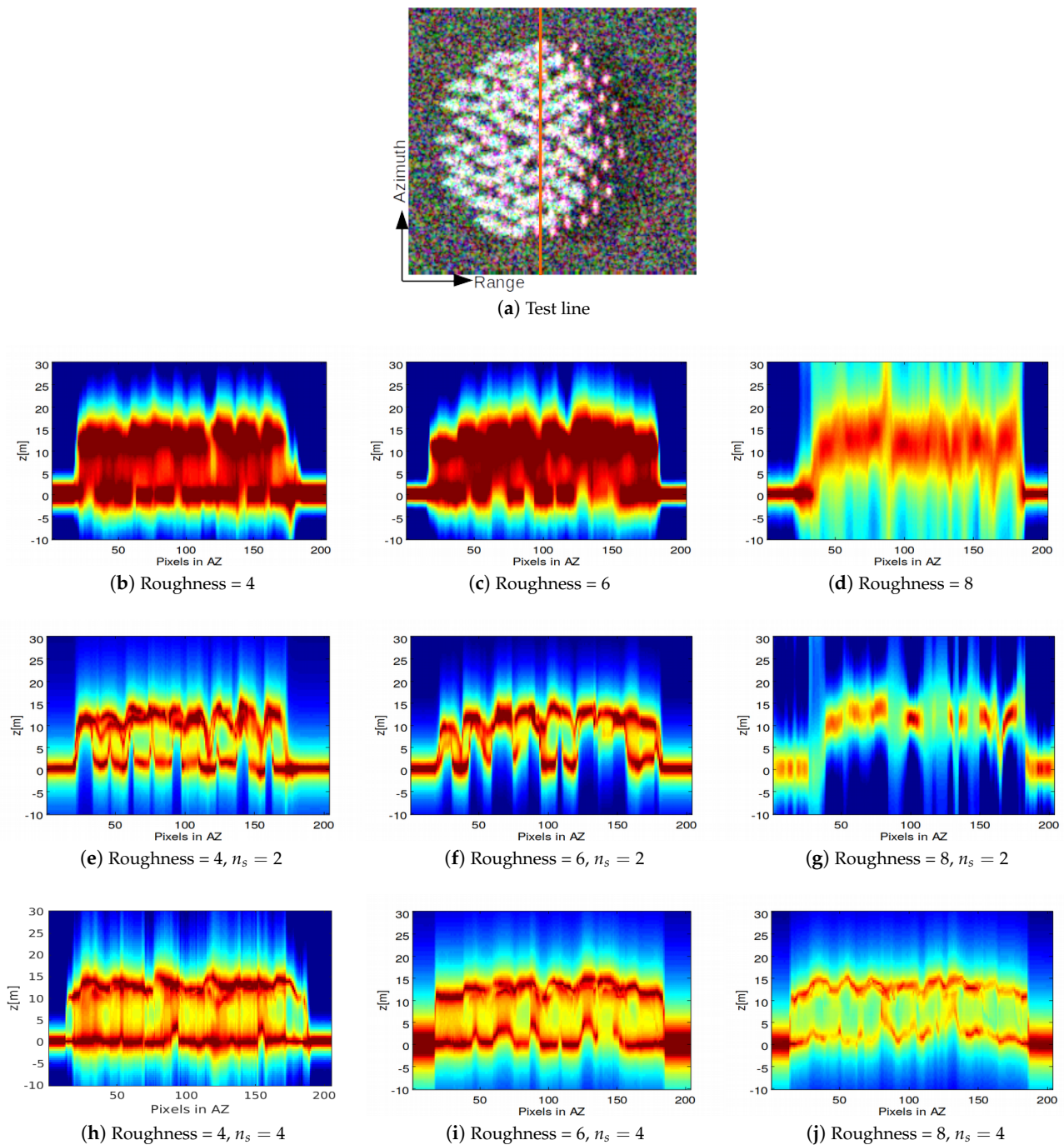
Figure 11. P-Capon and P-MUSIC tomograms with n_s = 2 and n_s = 4 over a test line for different ground roughness: P-Capon (b–d); and P-MUSIC (e–j).
