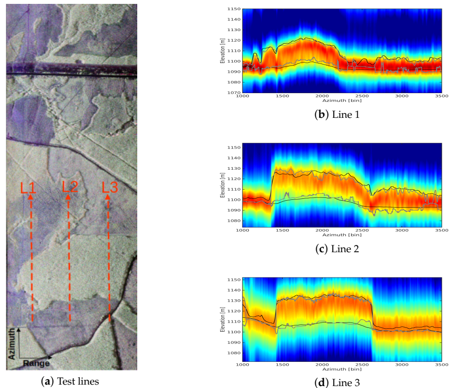
Figure 13. Ground topography and tree top heights estimated by the proposed tomographic approach. Background, P-Capon tomograms; gray line, estimated ground and tree top elevations; black line, LiDAR ground and tree top elevation estimates.
