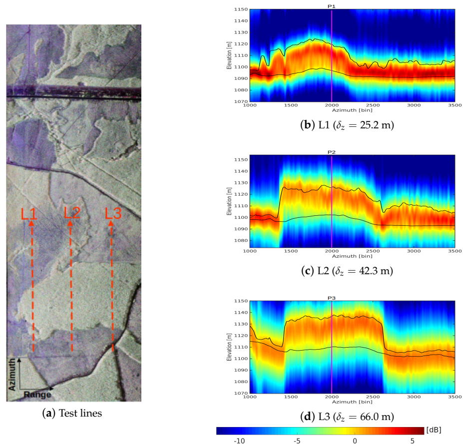
Figure 6. P-Capon tomograms for test lines located in near, mid and far range, respectively. The black line is the LiDAR ground and tree top elevation estimates.
