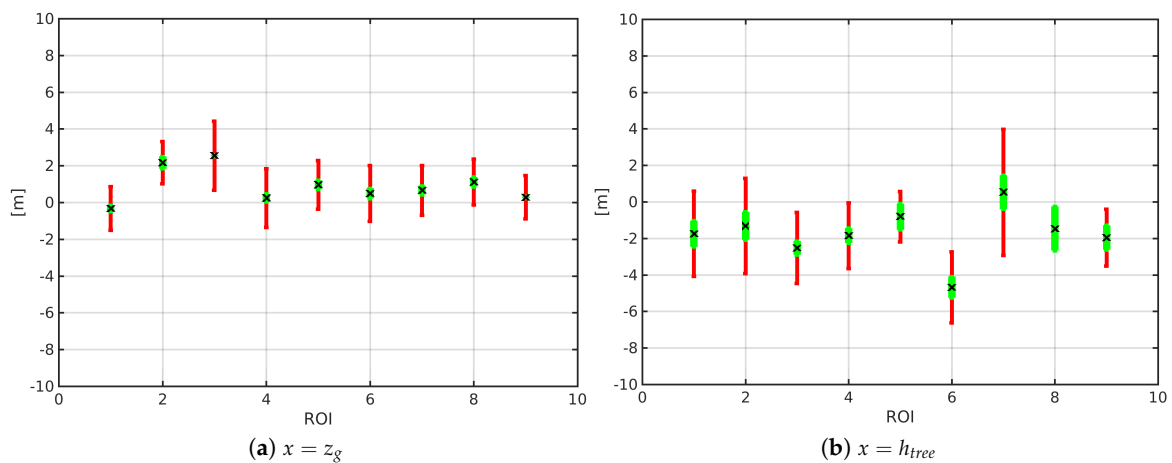
Figure 18. Statistical features of TomoSAR- and LiDAR-derived elevation estimates over different ROIs. The red bar has a length equal to 2\hat{\sigma}_{\Delta x_i} , the black cross mark indicates \hat{m}_{\Delta x_i} and the green bar has a length equal to 2\hat{\sigma}_{Lidar,i} , with i = 1, \dots, 9 .
