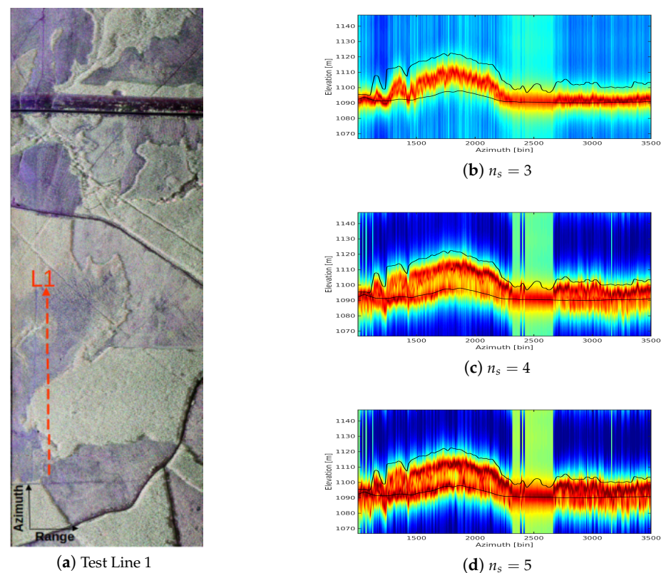
Figure 9. P-MUSIC tomograms with model order larger than 2. The black line is the LiDAR ground and tree top elevation estimates.
