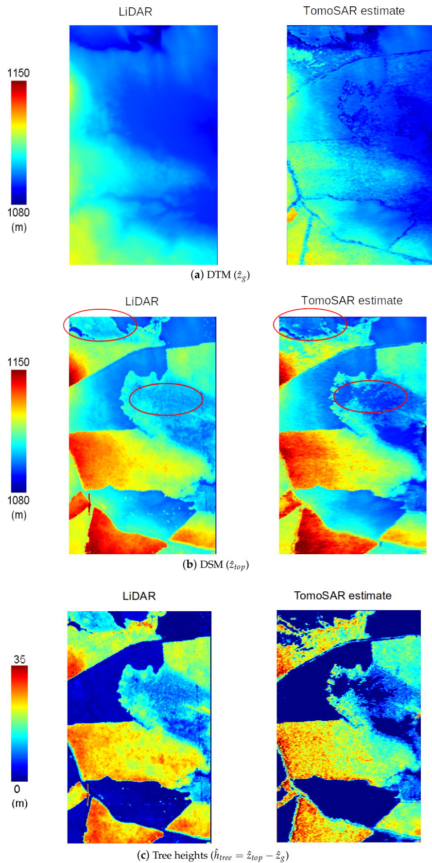
Figure 16. DSM, DTM and tree height maps estimated by the proposed tomographic technique and using LiDAR data.
