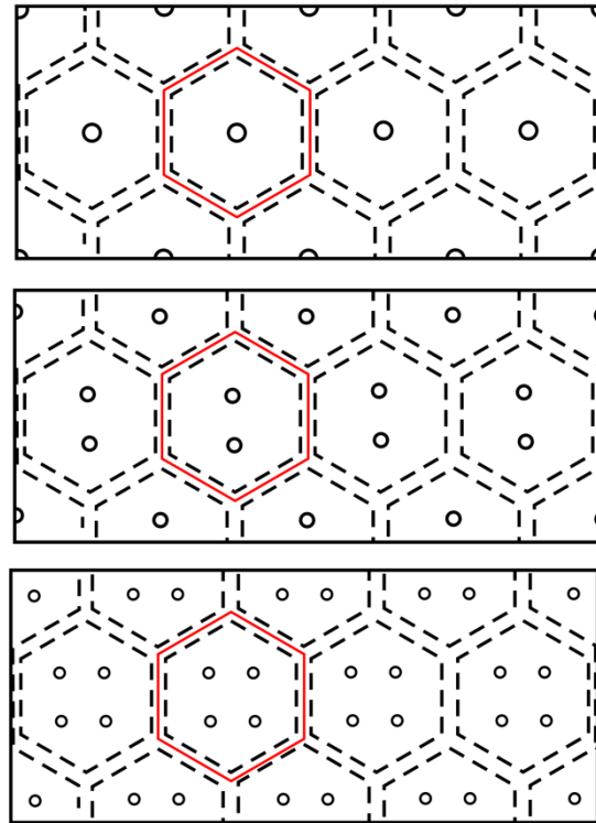
Fig. 11 Schematic of hexagonal sandwich panels with different pore diameters but fixed perforation ratio
