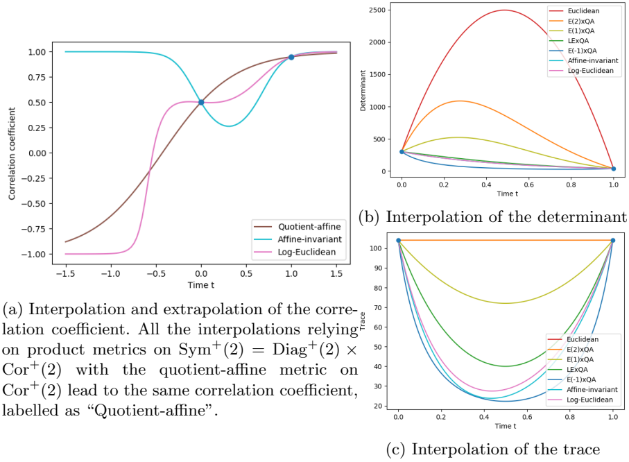
Fig. 1: Extrapolation and interpolation between the SPD matrices \Sigma_1 and \Sigma_2 using various Riemannian metrics. The metrics E(p)\times\text{QA} refer to the p -power-Euclidean metric on the diagonal part and the quotient-affine metric on the correlation part. When p tends to 0, the p -power-Euclidean metric E(p) tends to the log-Euclidean metric \text{LE} = E(0) .
