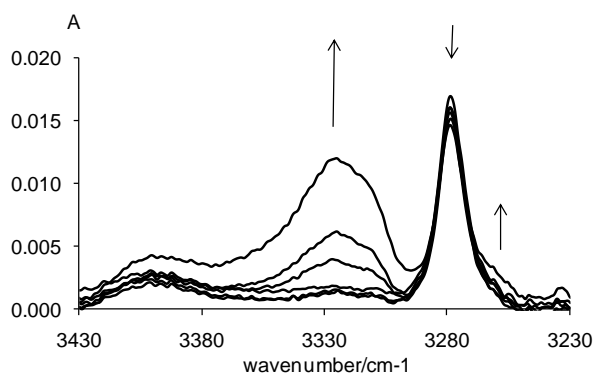
Figure 8. Infrared study of the reaction of [\text{RhI}(\text{PPh}_3)_2]_2 ( c = 3 \cdot 10^{-3} \text{ M} ) with \text{NHEt}_2 in \text{CH}_2\text{Cl}_2 (pathlength = 2.2 mm), after addition of \text{NHEt}_2 with the successive concentrations (3, 4.5, 6, 12, 18 and 30 \cdot 10^{-3} \text{ M} ).
