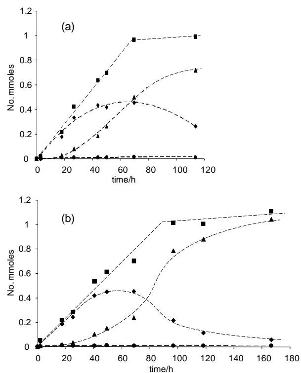
Figure 1. Kinetic profile of the \text{RhCl}_3 \cdot 3\text{H}_2\text{O} -catalyzed reaction between \text{PhNH}_2 and \text{C}_2\text{H}_4 : 1 (♦), 2 (▲),
