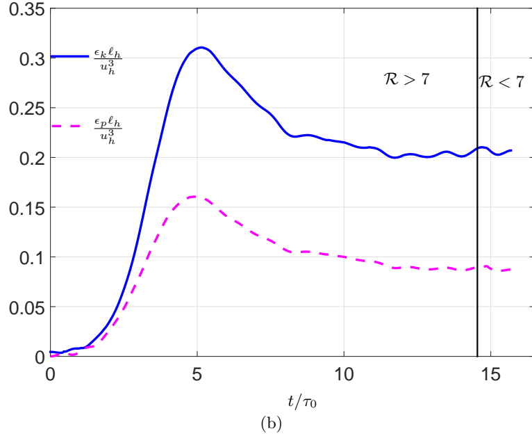
FIGURE 7. (a) Total energy dissipation \epsilon = \epsilon_k + \epsilon_p normalized by u_h^3/\ell_h as a function of time for four runs at different Fr . The vertical black segment indicates, for each run, the bound between times at which \mathcal{R} > 7 and later times at which \mathcal{R} < 7 . (b) The viscous dissipation and diffusive dissipation normalized analogously for run R49F0.1 with the same bound indicated on the plot.
