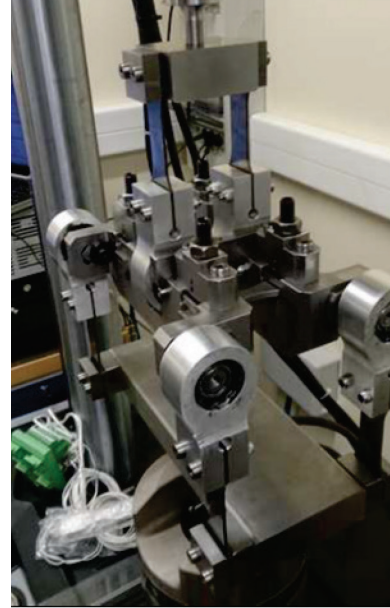
Figure 1 Specimen geometry (a). Thickness 2 mm. Dimensions in mm. Bending test bench (b)
