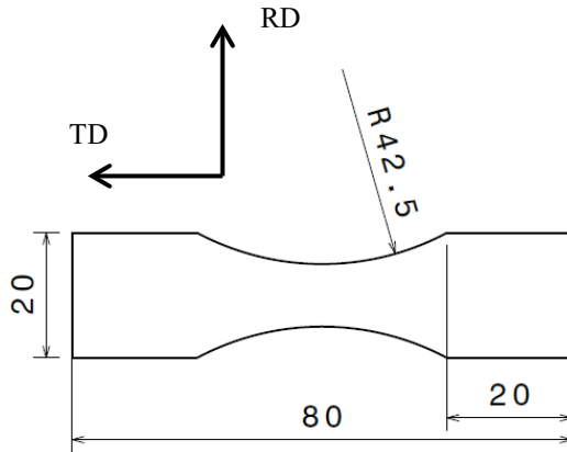
Figure 1 Specimen geometry (a). Thickness 2 mm. Dimensions in mm. Bending test bench (b)
