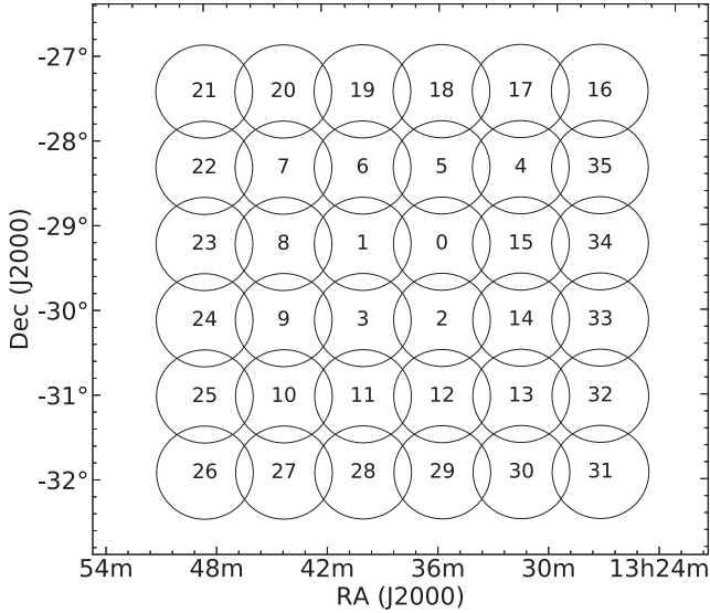
Figure 1. Position and beam number of the ASKAP 6^\circ \times 6^\circ square footprint centred on \alpha_A = 13^h37^m54^s and \delta_A = -29^\circ43'50'' .
