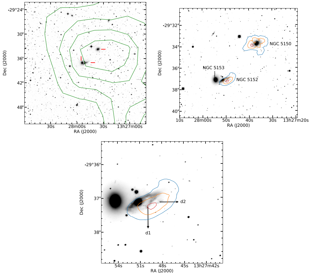
Figure 19. Top left: H I intensity contours (green) from the HIDEEP survey ( V_{\text{opt}} = 3195\text{--}4604\text{ km s}^{-1} ) overlaid on to the DSS2r image. The contour levels are 0.05, 0.1, 0.15, and 0.2\text{ Jy beam}^{-1} . The positions of NGC 5150, NGC 5152, and NGC 5153 are indicated by the red markers. Top right: Zoom in to the NGC 5150 subgroup region with H I column density contours overlaid on to the DECAM image (refer the contour levels in Fig. 9). Bottom: Zoom in to show the interacting pair, NGC 5152 and NGC 5153, where the tidal dwarf candidates are labelled as d1 and d2 (see Weilbacher et al. 2000).
