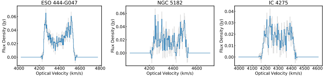
Figure 6. Examples of spectra of individual sources derived by SOFIA. Local RMS is shaded in grey. Note. This figure is published in its entirety as Supporting Information with the electronic version of the paper. A portion is shown here.
