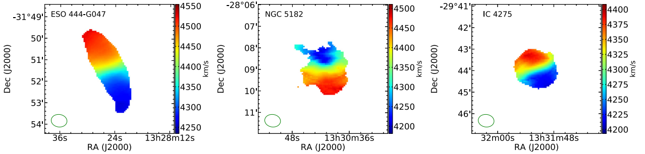
Figure 10. Examples of velocity field maps of individual sources, where only pixels above 3 \times N_{\text{H I, sen}} are plotted. The synthesized beam of 45 arcsec \times 35 arcsec is plotted at the bottom left corner of each sub-plot. Note. This figure is published its entirety as Supporting Information with the electronic version of the paper. A portion is shown here.
