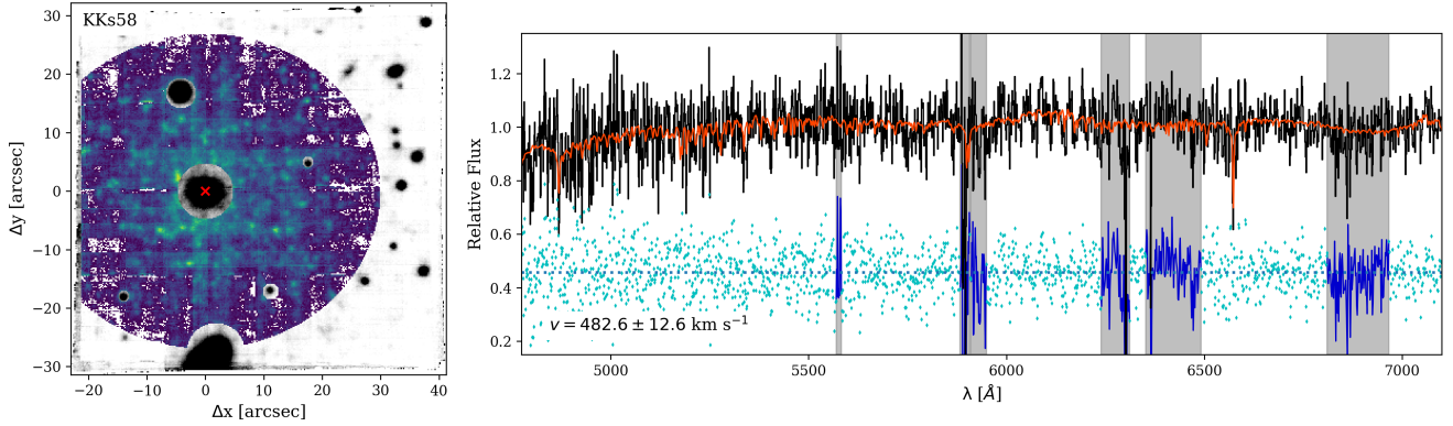
Fig. 4. Extraction of the KKs58 galaxy spectrum. Left: white-light image of KKs58, created by collapsing the MUSE cube along the spectral axis ( 10'' \approx 160 pc). The position of the NSC is marked by the red cross. We show the mask that is used for the extraction of the integrated galaxy spectrum in green-blue colours while the masked pixels are shown with are in black and white. Right: pPXF fit to the normalised integrated spectrum of KKs58. The input spectrum is shown in black and the best-fitting combination of MILES SSP models is shown in red. The blue points indicate the residual, shifted to 0.5 for visibility. Masked regions with strong sky residual lines appear as grey-shaded. We only use the spectral range from 4500 to 7100 Å because the spectrum is heavily contaminated by sky residual and telluric lines at larger wavelengths.
