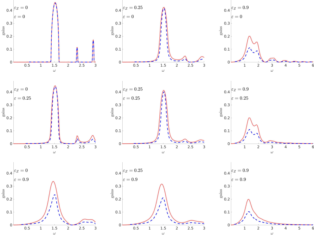
FIG. 5. Sample and mean MI gains for a simple random walk process and \bar{\lambda} = 1 and \delta\lambda_n uniform in [-1, 1] . Color code is the same as Fig. 2
