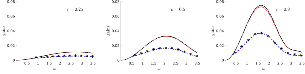
FIG. 3. Same as Fig. 2, with Z_n as in Eq. (14) (Poisson model). The parameter \varepsilon is indicated in the panels.
