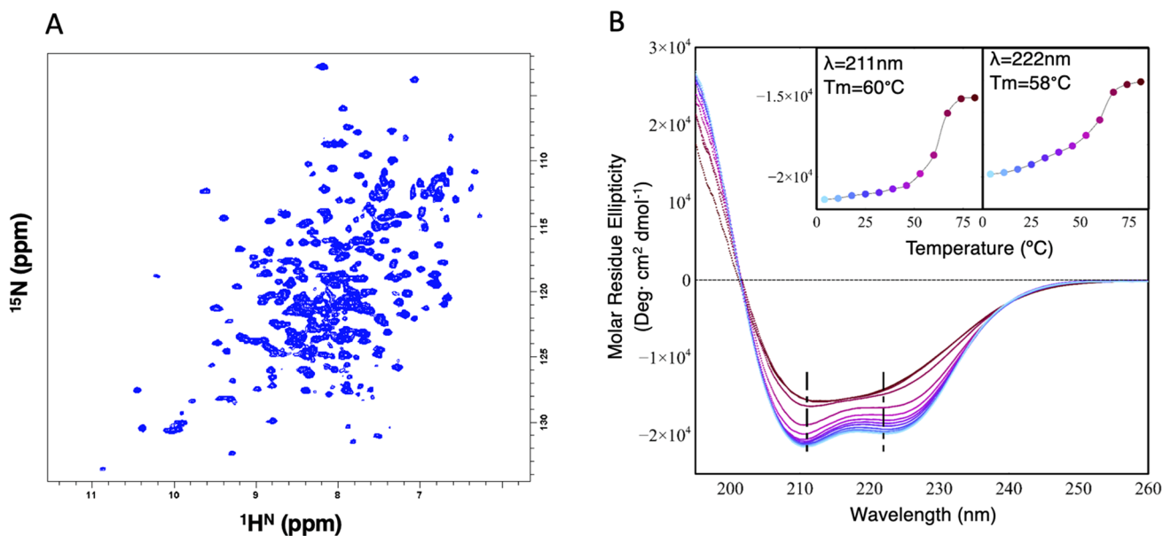
Fig. 1 FhuF is a folded protein. a 2D ^1\text{H}/^{15}\text{N} TROSY-HSQC spectrum of ^{15}\text{N}/^{13}\text{C} -labeled FhuF collected at 305 K on a Bruker Avance III 800 MHz spectrometer. The resonance map has the typical fingerprint of a folded protein with large chemical shift dispersion. b CD spectra
