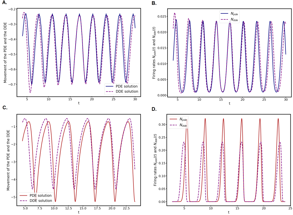
Figure 7: Comparison between the maximum point of the PDE (1.4) and the DDE (5.4); (A.) Setup 5.1 with b = -45 ; (B.) comparison of the firing rates N(t) and \mathcal{N}(c(t)) in Setup 5.1 with b = -45 ; (C.) Setup 5.2 with b = -35 ; (D.) comparison of the firing rates N(t) and \mathcal{N}(c(t)) in Setup 5.2 with b = -35 .
