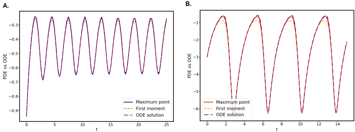
Figure 5: Comparison between the maximum point and first moment of the PDE (1.4) and the ODE (5.3); (A.) Setup 5.1 with b = -45 ; (B.) Setup 5.2 with b = -35 .
