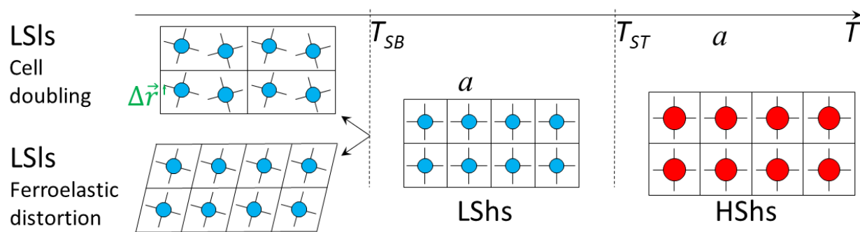
Figure 7 Representation of the sequence of phases with a non-symmetry-breaking spin transition at T_{ST} from HSs to LShs and a symmetry-breaking phase transition at T_{SB} from LShs to LSIs. A spin transition occurs with mainly HS molecules above and LS below. The symmetry breaking may have various nature, like cell doubling or ferroelastic distortion, and results in atomic motions \Delta\vec{r} , and motions or torsions of ligand, solvent or counter ions.
