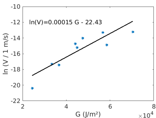
FIG. 18. Creep data of high density polyethylene, from Yoda et al. [17] , figure 4.
