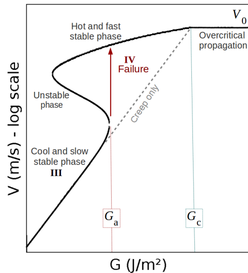
FIG. 2. Modelled crack velocity as a function of energy release rate, as per Eqs. (1) and (2). Stages III and IV correspond to the one labelled in Fig. 1. As explained in the text, stages 0, I and II are here not covered. In our model, the failure occurs when the cracks becomes hot enough, that is, when \Delta T \sim T_0 . The dashed line corresponds to a cold case \Delta T \ll T_0 in Eq. (1).
