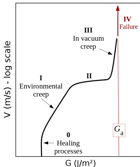
FIG. 1. Summary of the different forward crack velocity regions observed in experimental velocity curves. After Fracture of Brittle Solids , Lawn [5]
