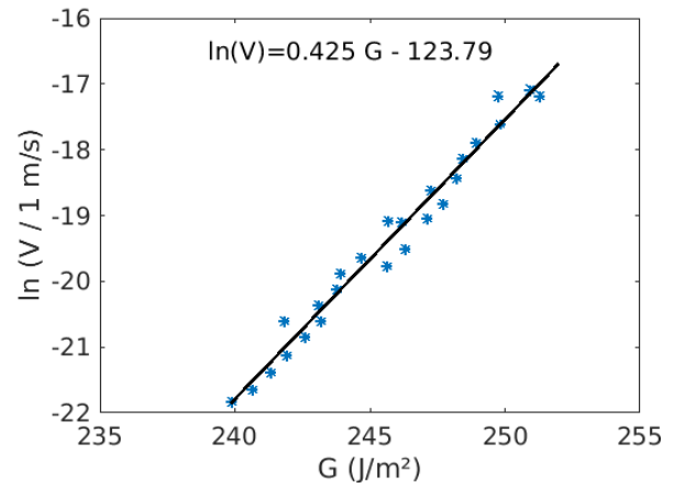
FIG. 12. Creep data cement in water, from Wang et al. [11] , figure 4a.
