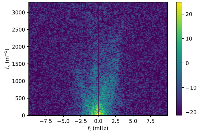
Figure 13. Secondary spectrum of J1757–5322 showing a clear scintillation arc, which we observe to change in curvature with the binary phase. The colour scale represents the power (in arbitrary units) in each pixel.
