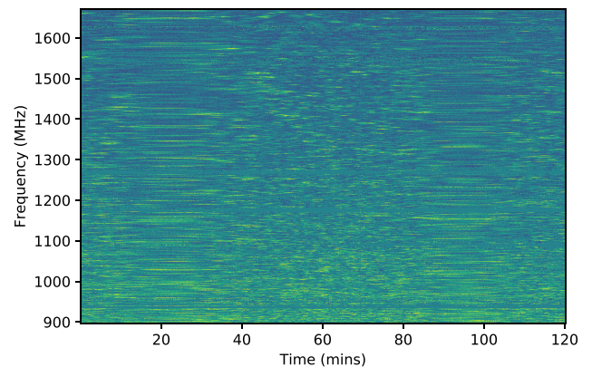
Figure 10. Dynamic spectrum of the double pulsar obtained from a 2-h observation of the pulsar. The stretching and squeezing of the blobs of power are caused due to the pulsar’s orbital motion.
