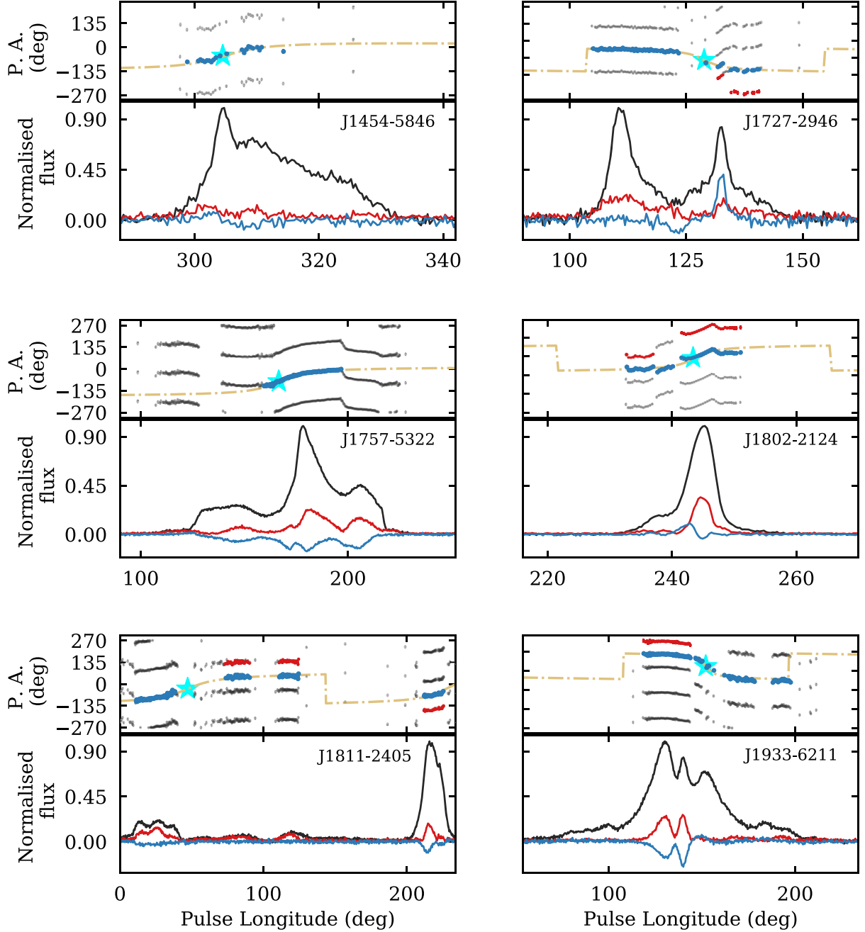
Figure 6. Pulse profiles for relativistic binary pulsars, where we try to model the PA with a Rotating Vector Model (RVM). The data properties and panel descriptions are the same as Fig. 1. The subpanels showing the PAs also show the best-fitting rotating vector model as a dash-dotted brown line. The black points in the panel are the original PA points – now made semitransparent for clarity. The blue ones are the points that are considered for the RVM fitting. The red points are the original locations of some PA points that had to be shifted by 90 deg to account for an orthogonal polarized mode transition, or shifted by 180 deg for fitting convenience. The cyan star is the best-fitting position of (\phi_0, PA_0) – see the text for more details.
