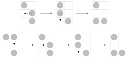
Figure 26. Subroutines used when c_2 is to the bottom-right of c_1 .
