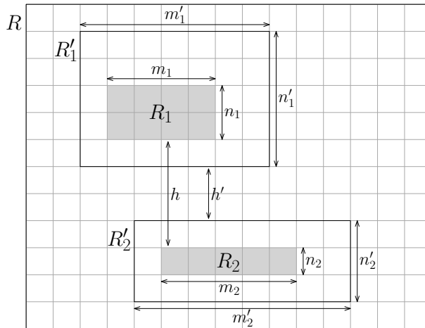
Figure 14. Illustration of R , R_1 , R_2 , R'_1 , R'_2 .
