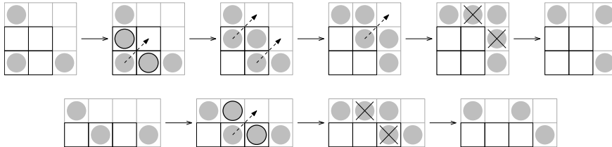
Figure 6. Subroutines used to flip an even ‘L’. The bottom subroutine is only used if both sides are even.
