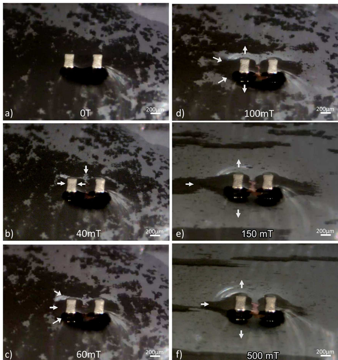
Figure S5: Snapshots taken during the deposition of a dilute suspension of Co NRs ([Co] ~ 20 g/L) on top of two Ni blocks ( 200\ \mu\text{m} ( L ) x 500\ \mu\text{m} ( W ) x 150\ \mu\text{m} ( T )) and placed in an external magnetic field of a) 0, b) 40 mT, c) 60 mT, d) 100 mT, e) 150 mT and f) 500 mT (Video S1). The white arrows are guide to the eye for the Co NR motion. For clarity they are only presented for the left-hand side Ni block.
