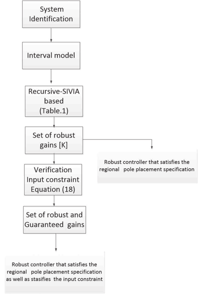
FIGURE 3 Overall framework to obtain the set of robust and guaranteed gains [Colour figure can be viewed at wileyonlinelibrary.com ]
